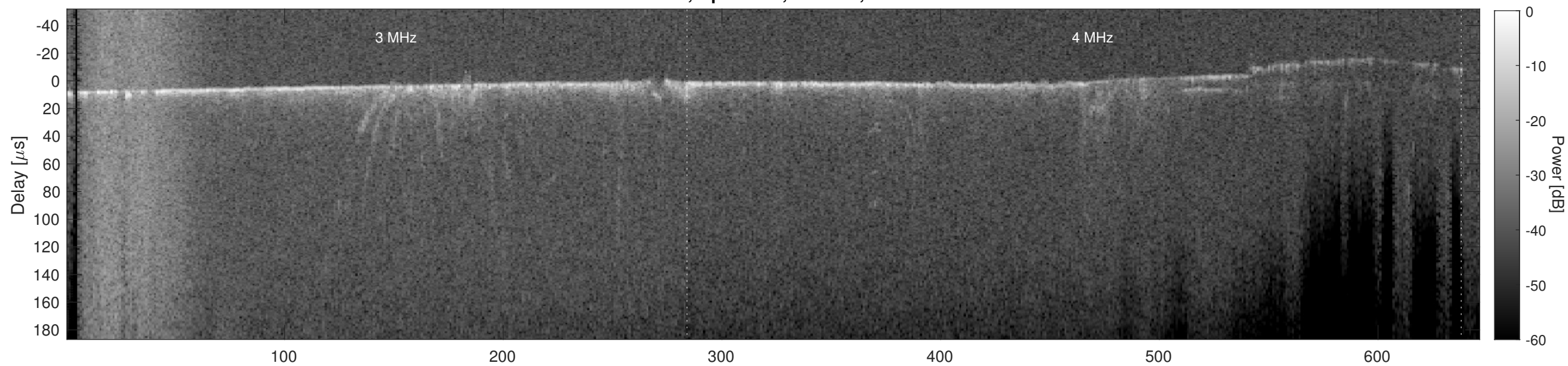
Orbit 22373, Cluttergram
