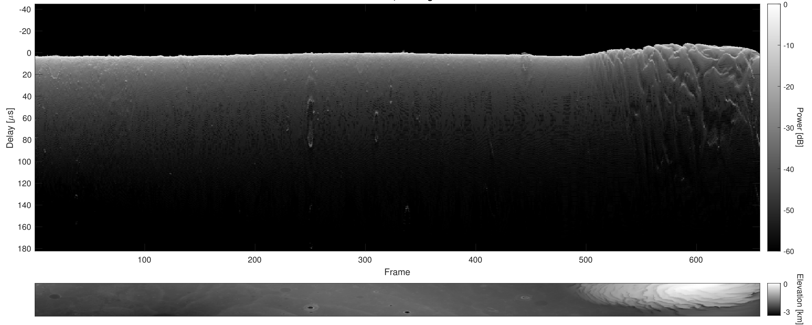
Orbit 22374, Cluttergram
