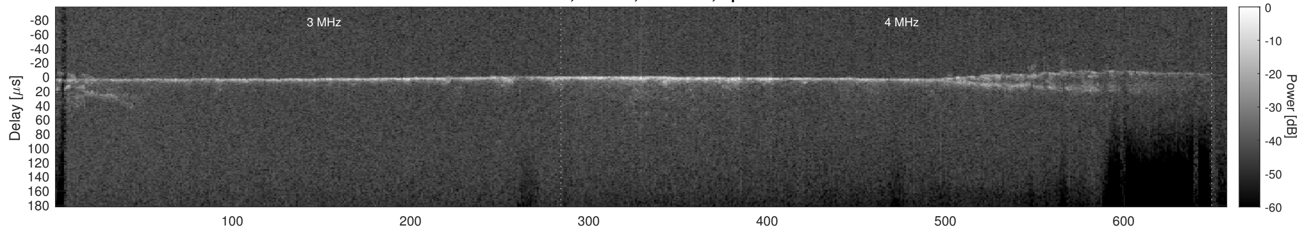
Orbit 22374, Cluttergram
