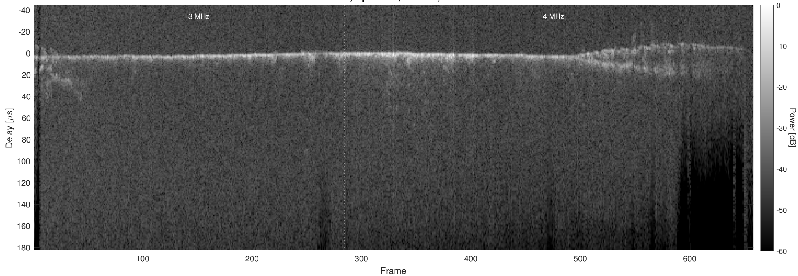
Orbit 22374, Optimized, Window, Channel 2
