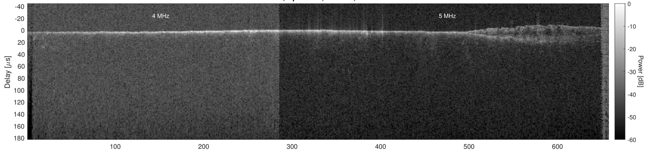
Orbit 22374, Optimized, Window, Channel 2
