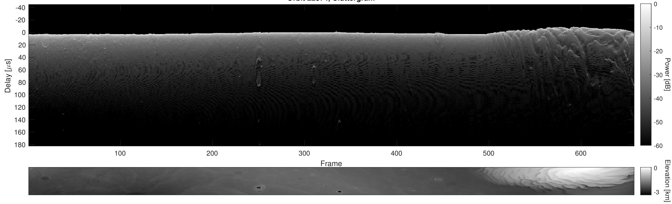
Orbit 22374, Cluttergram
