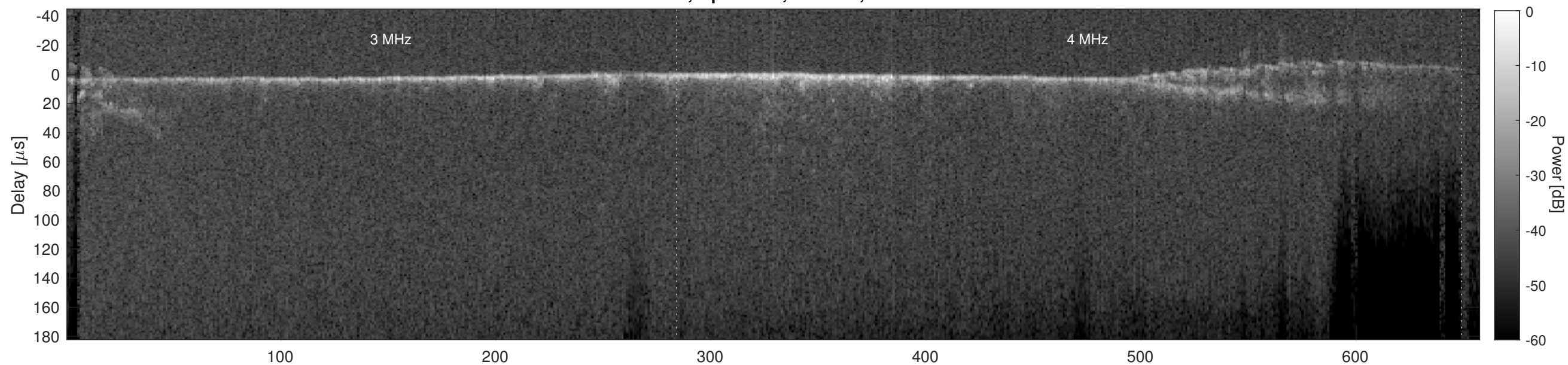
Orbit 22374, Cluttergram
