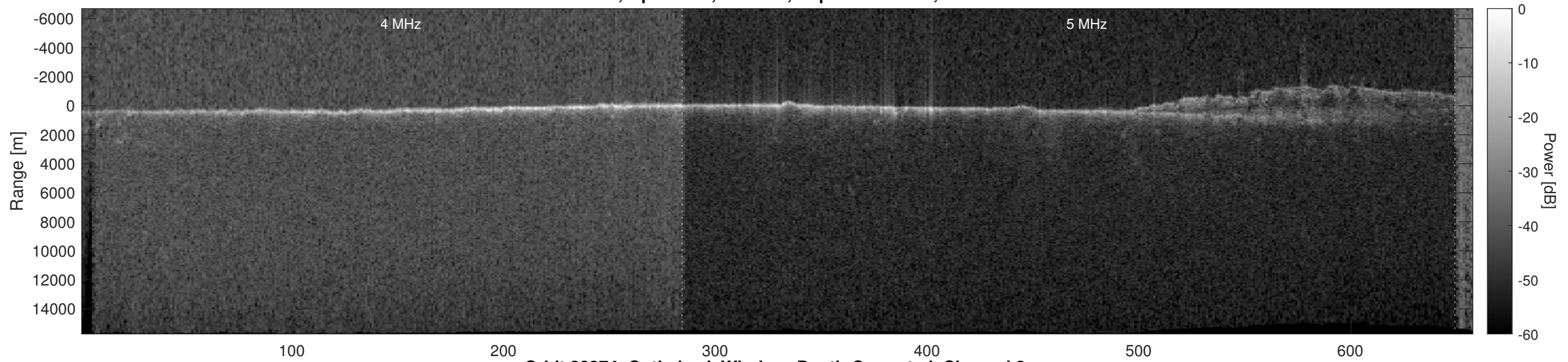
Orbit 22374, Optimized, Window, Depth-Corrected, Channel 2
