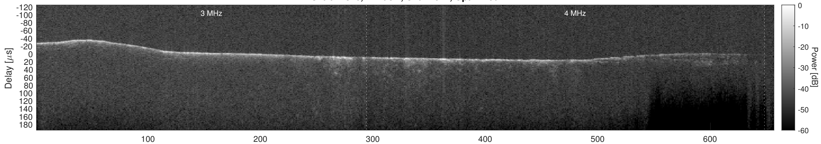
Orbit 22376, Cluttergram
