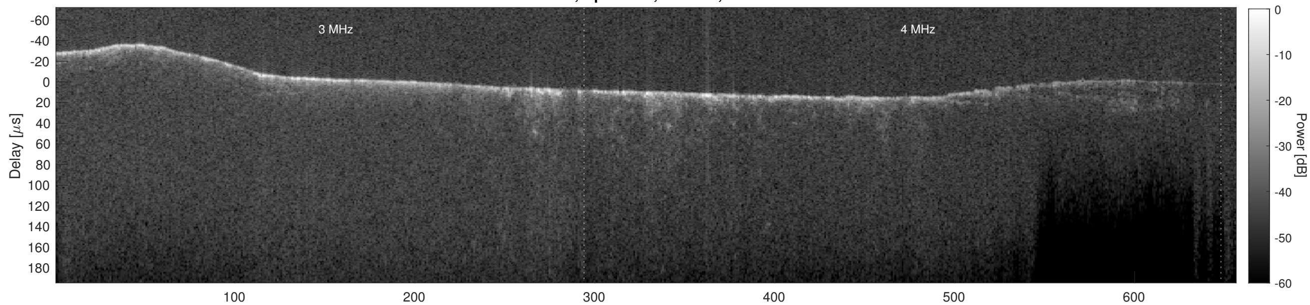
Orbit 22376, Cluttergram
