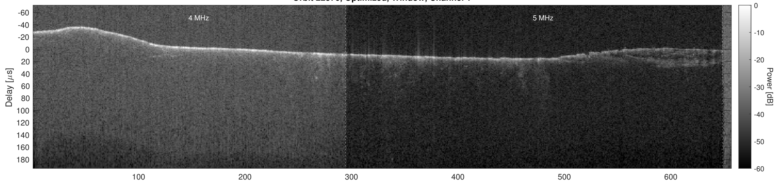
Orbit 22376, Optimized, Window, Channel 2
