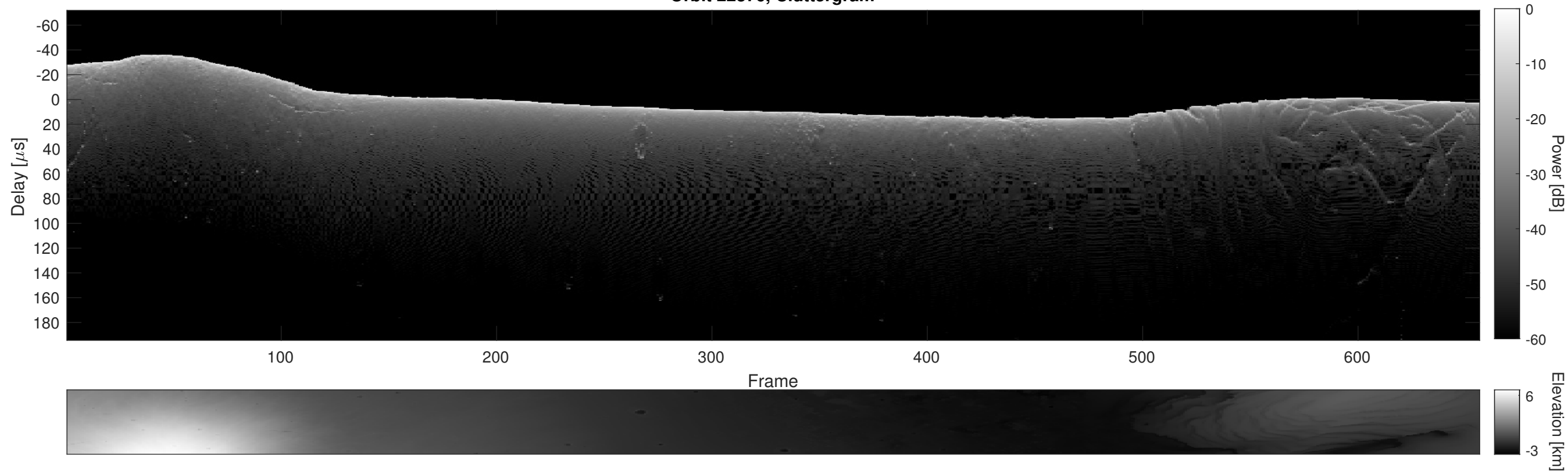
Orbit 22376, Cluttergram
