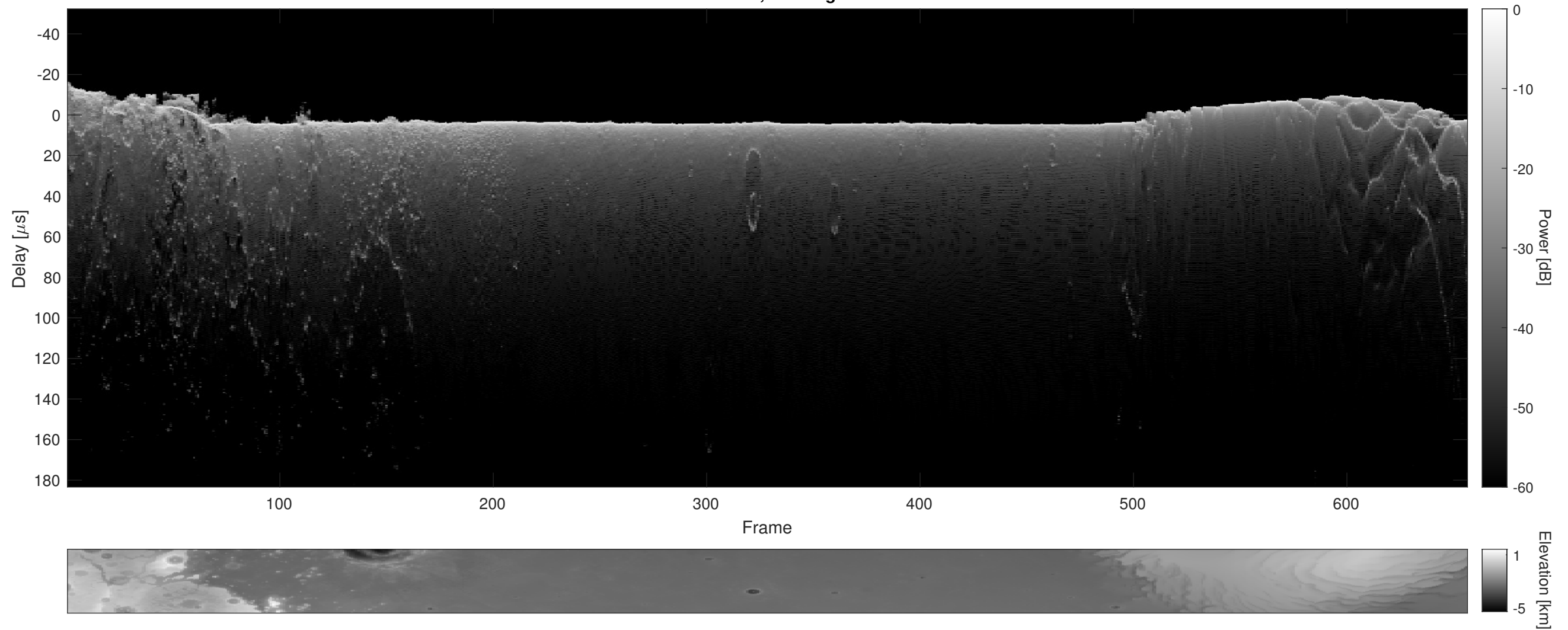
Orbit 22378, Cluttergram
