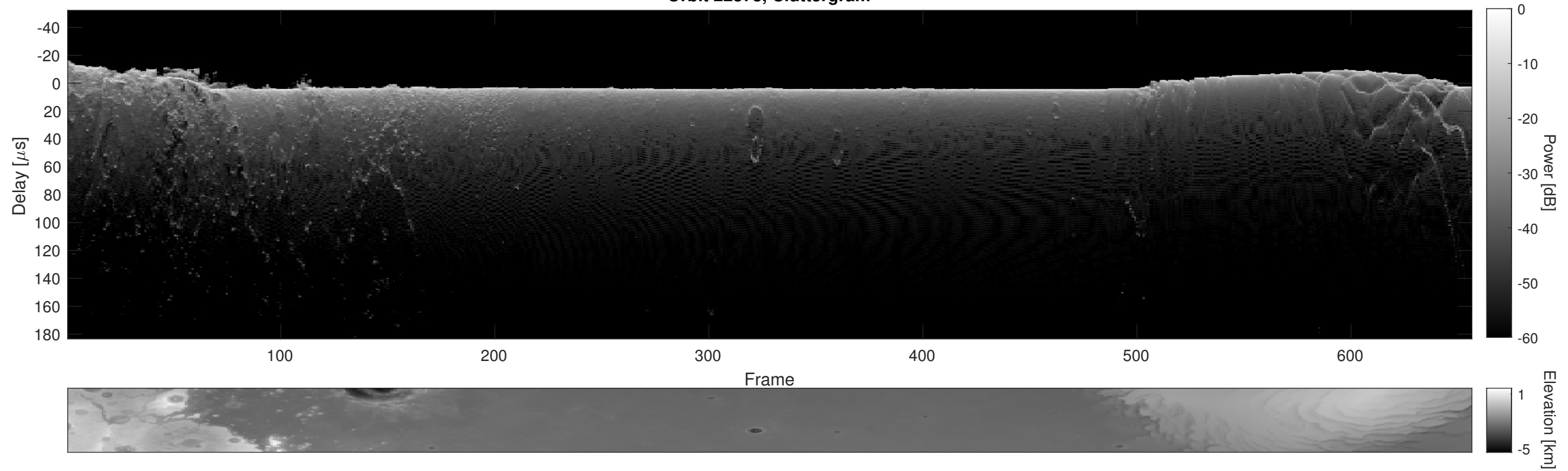
Orbit 22378, Cluttergram
