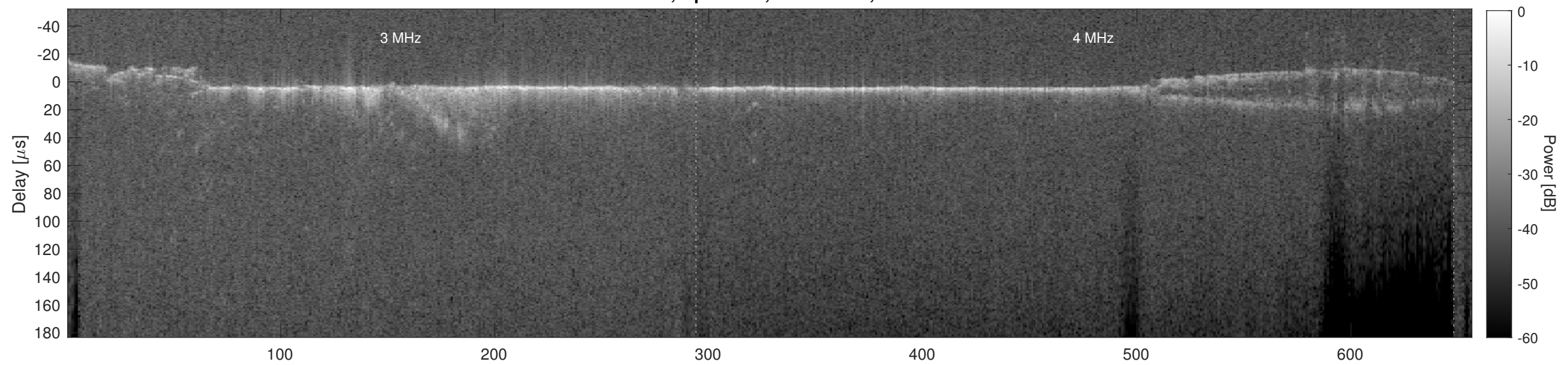
Orbit 22378, Cluttergram
