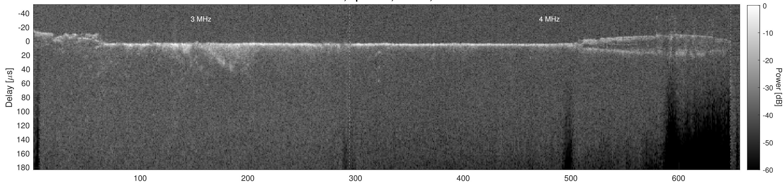
Orbit 22378, Cluttergram
