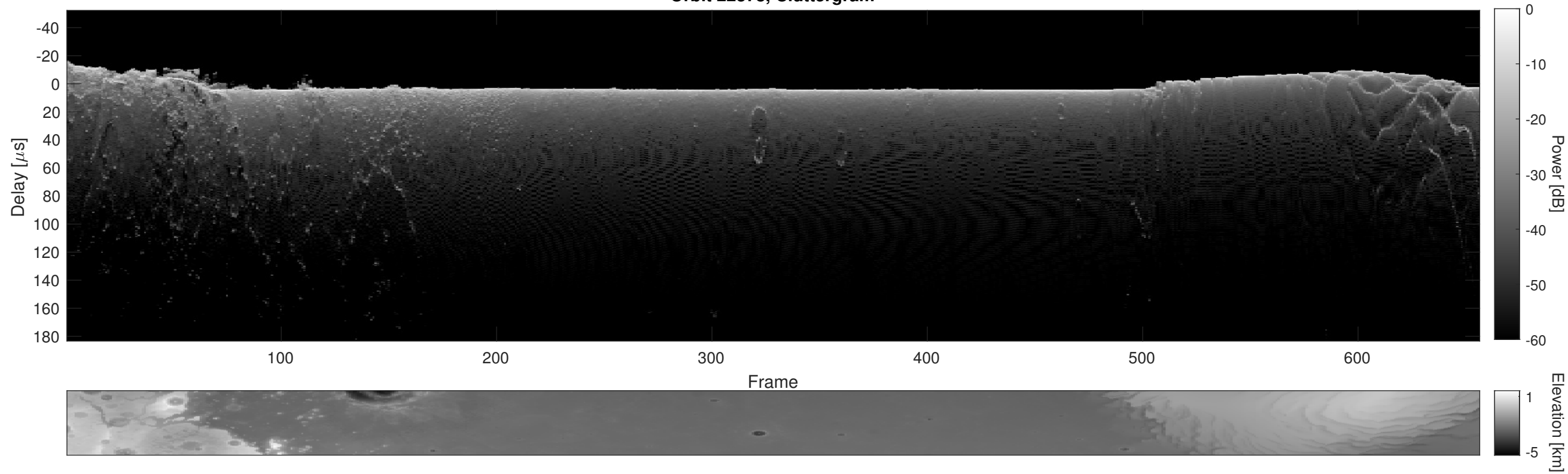
Orbit 22378, Cluttergram
