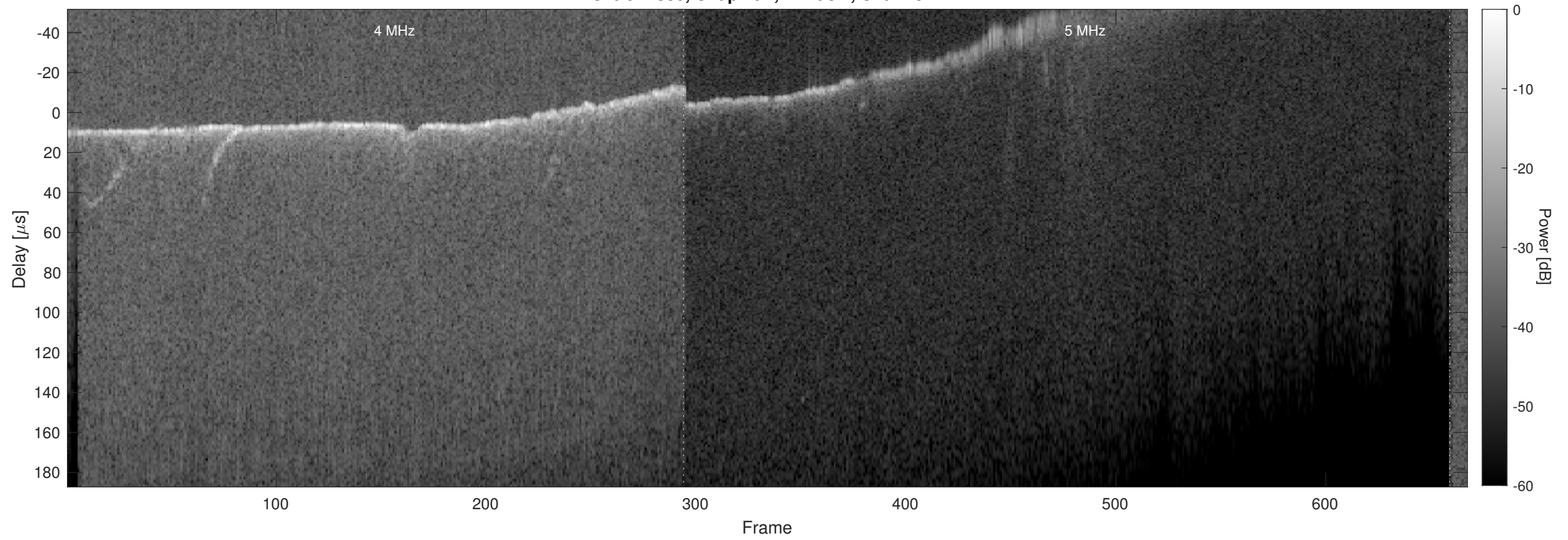
Orbit 22380, Chapman, Window, Channel 2
