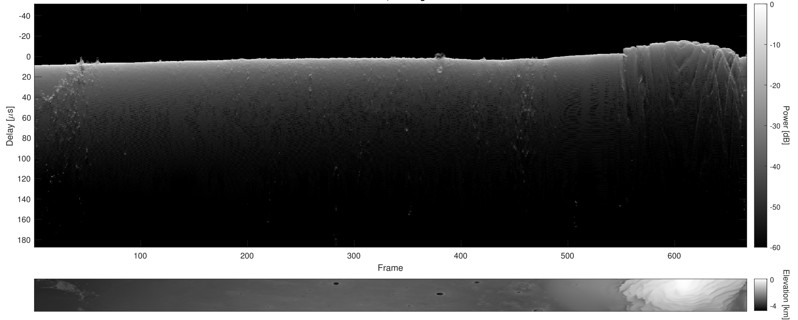
Orbit 22380, Cluttergram
