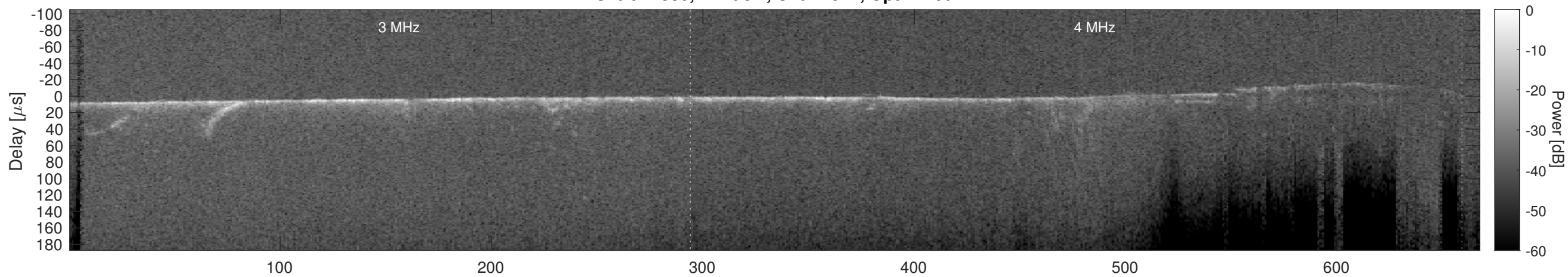
Orbit 22380, Cluttergram
