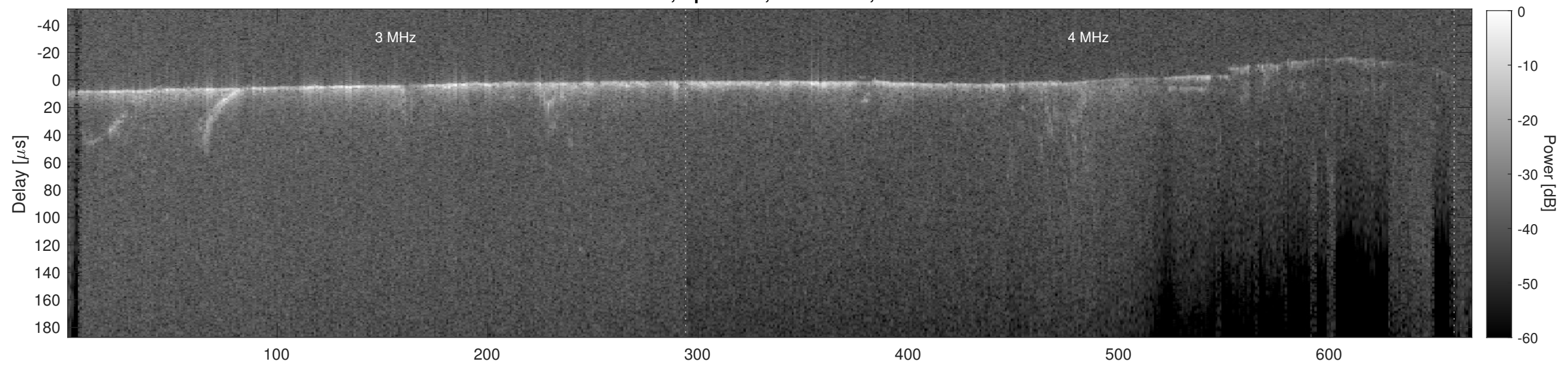
Orbit 22380, Cluttergram
