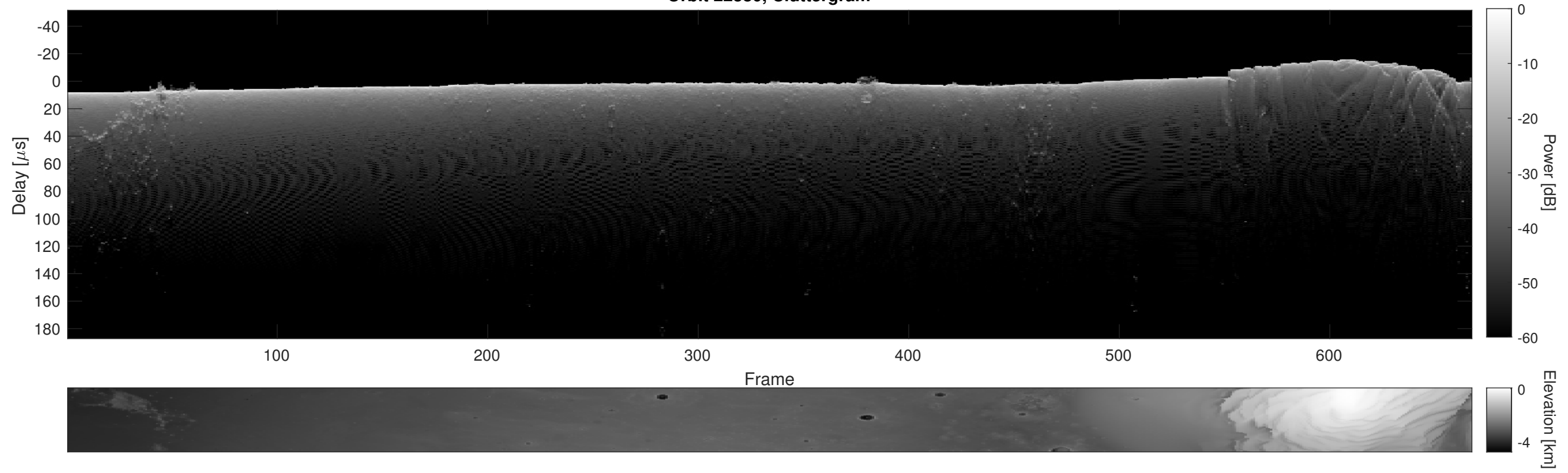
Orbit 22380, Cluttergram
