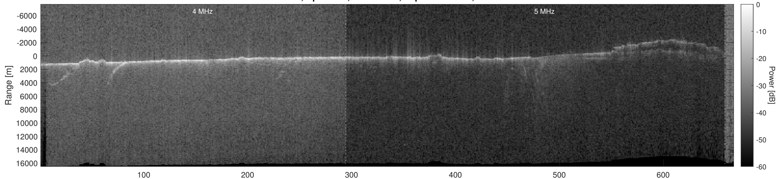
Orbit 22380, Optimized, No Window, Depth-Corrected, Channel 2
