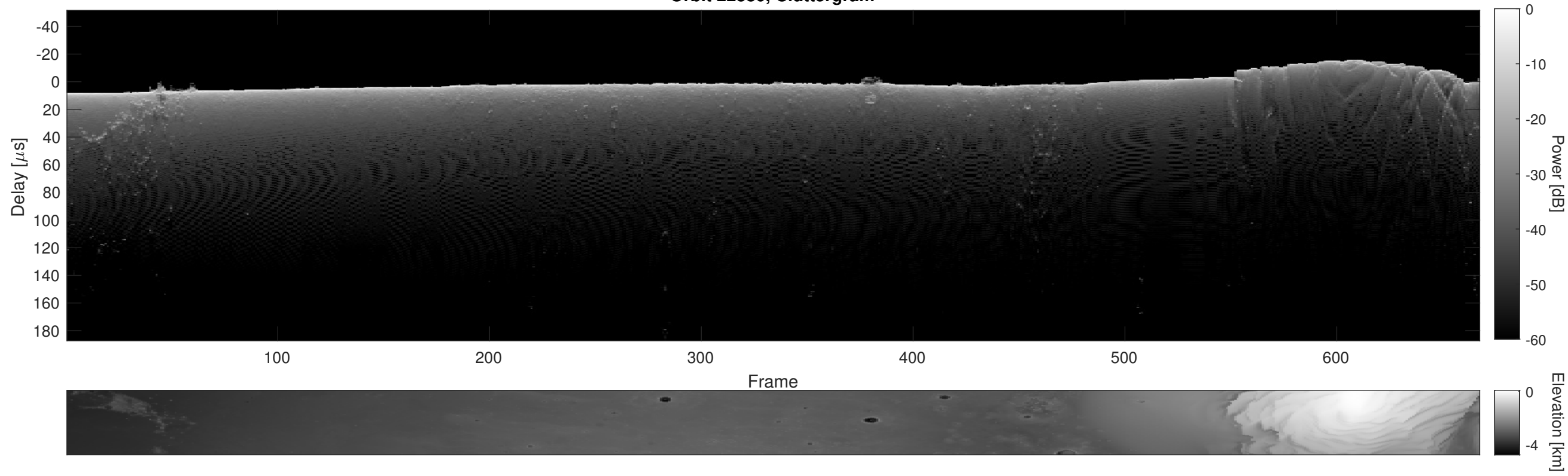
Orbit 22380, Cluttergram
