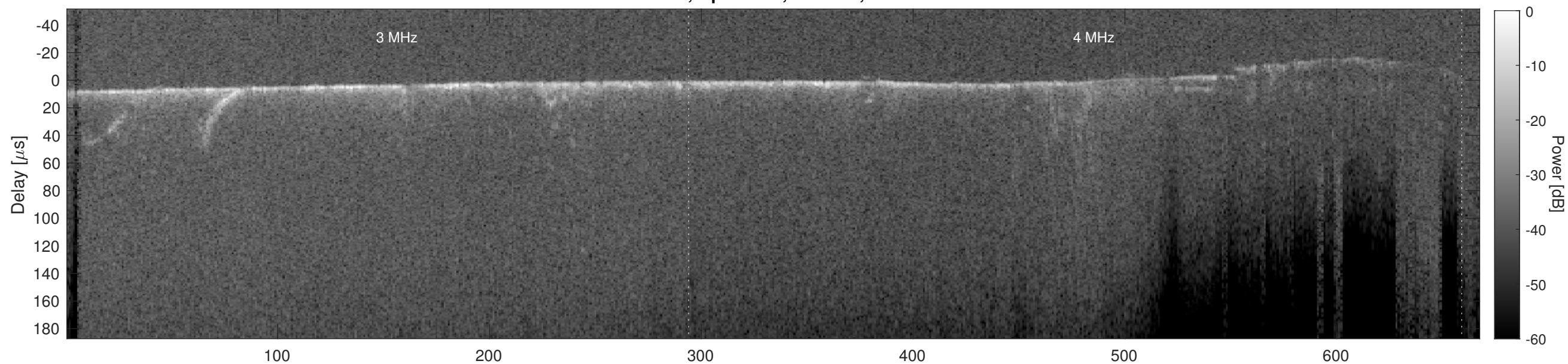
Orbit 22380, Cluttergram
