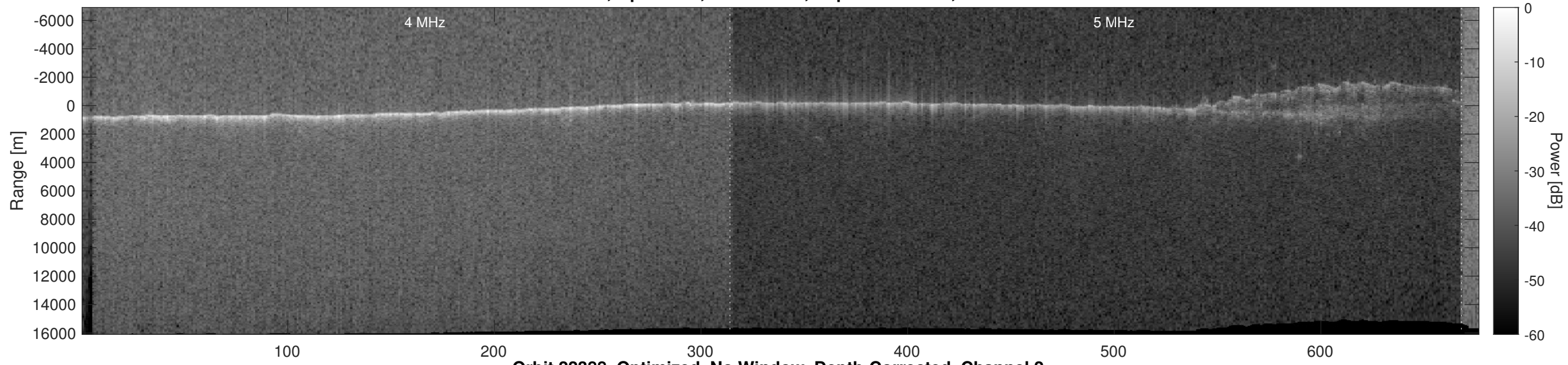
Orbit 22388, Optimized, No Window, Depth-Corrected, Channel 2
