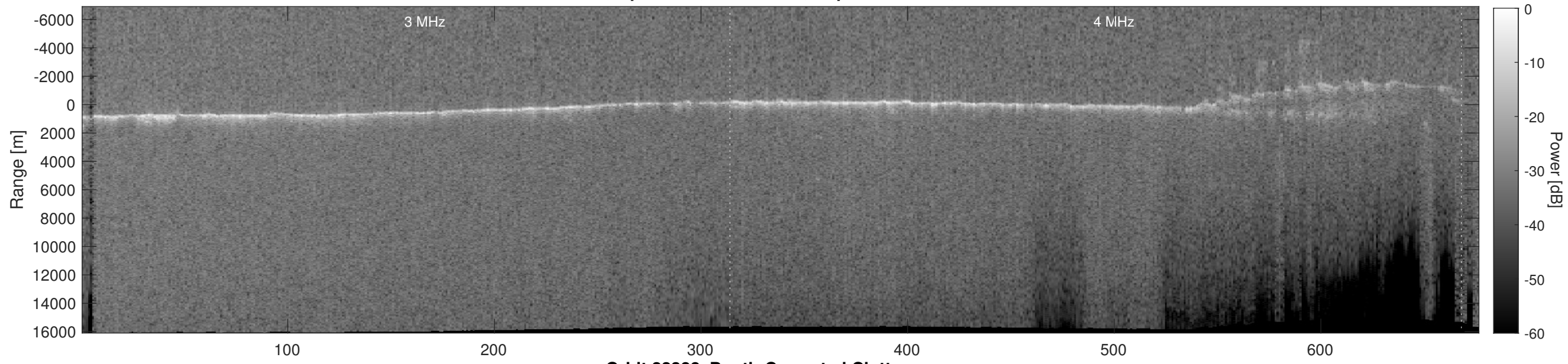
Orbit 22388, Depth-Corrected Cluttergram
