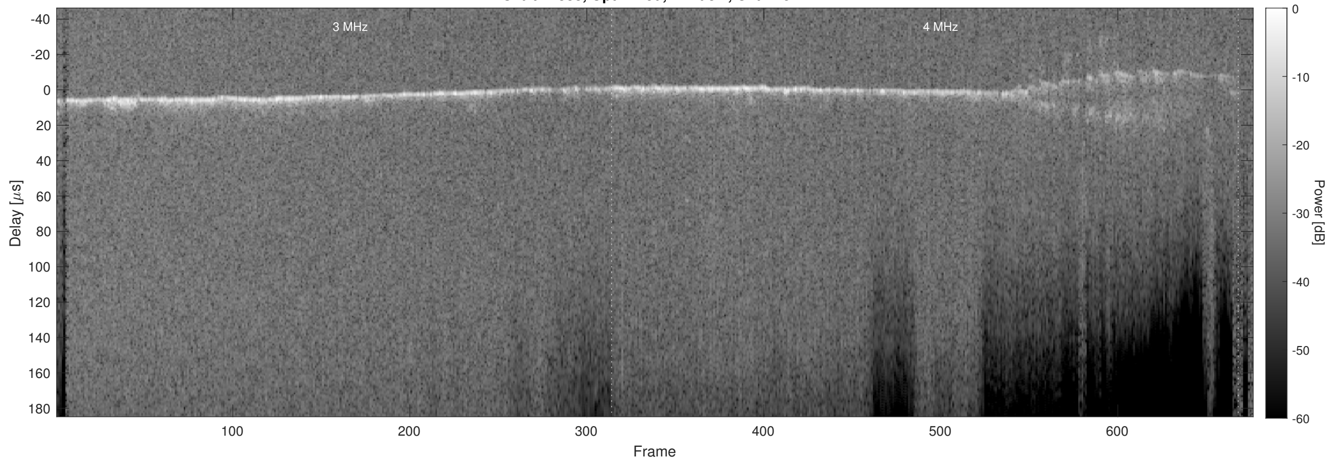
Orbit 22388, Optimized, Window, Channel 2
