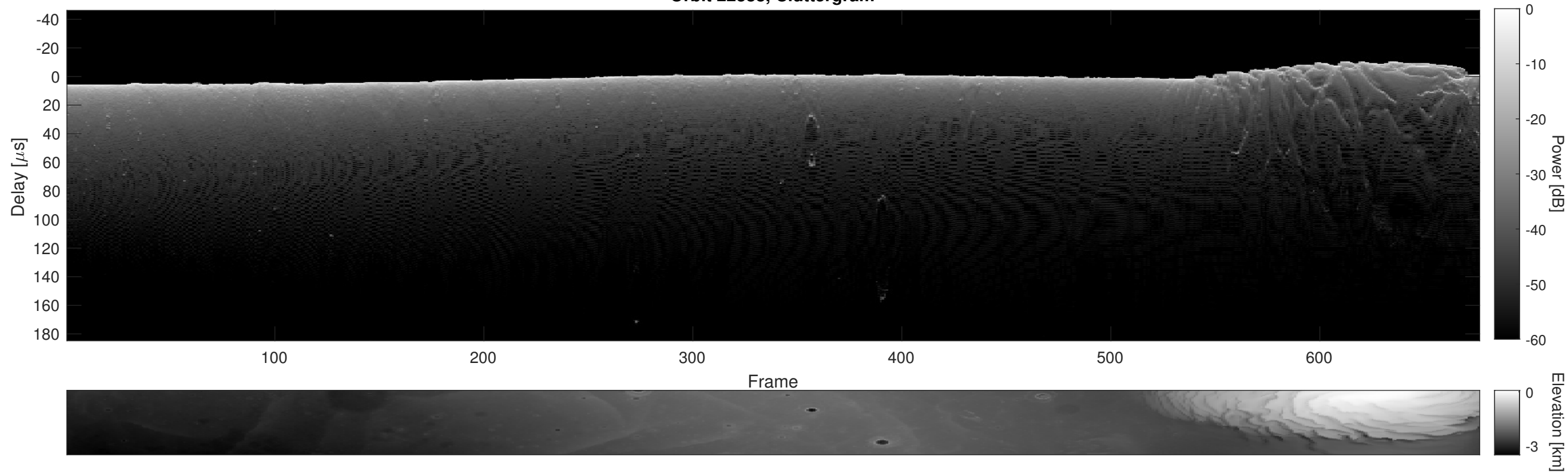
Orbit 22388, Cluttergram
