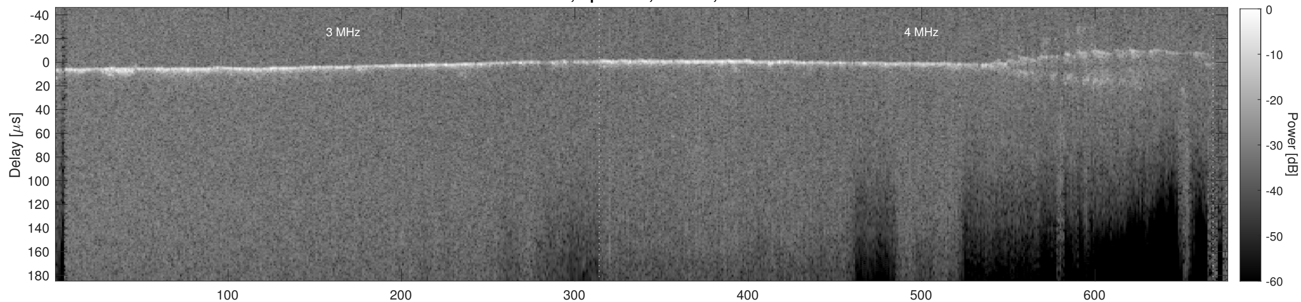
Orbit 22388, Cluttergram
