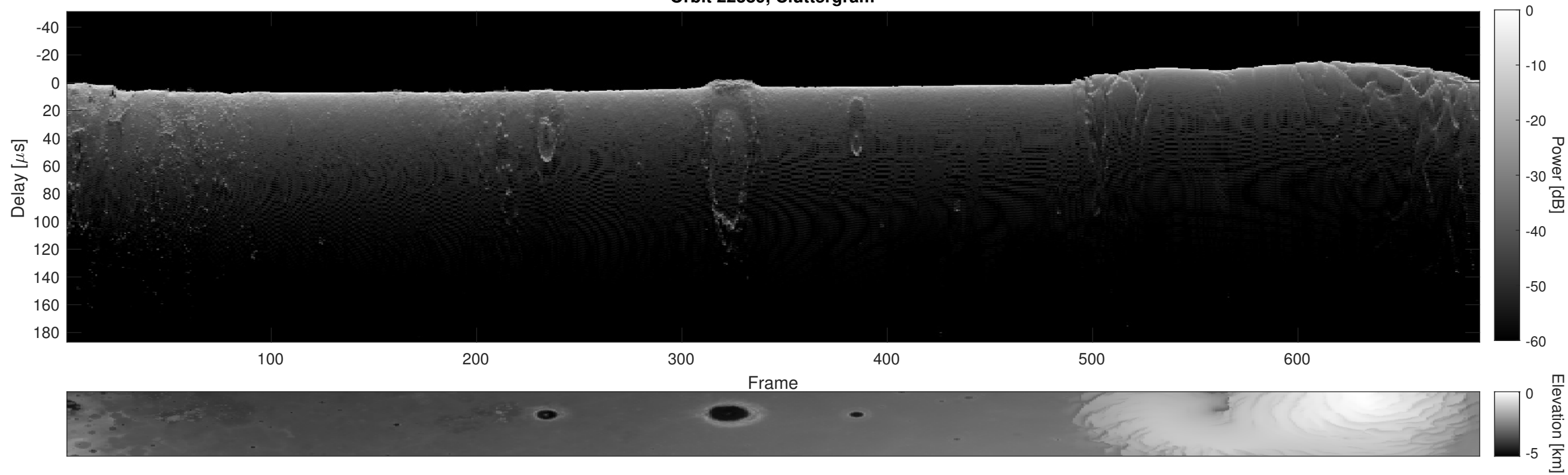
Orbit 22389, Cluttergram
