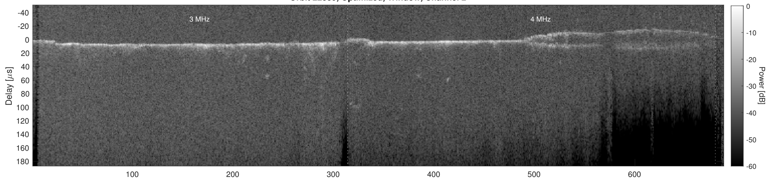
Orbit 22389, Cluttergram
