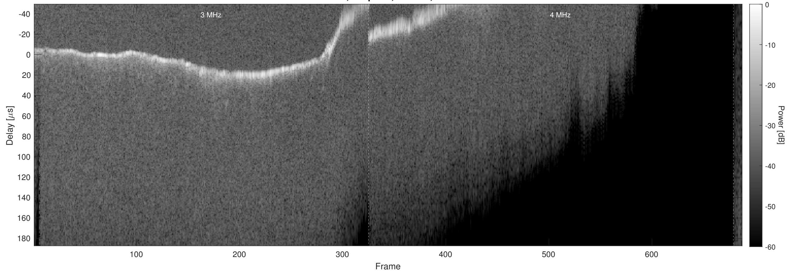
Orbit 22393, Chapman, Window, Channel 2
