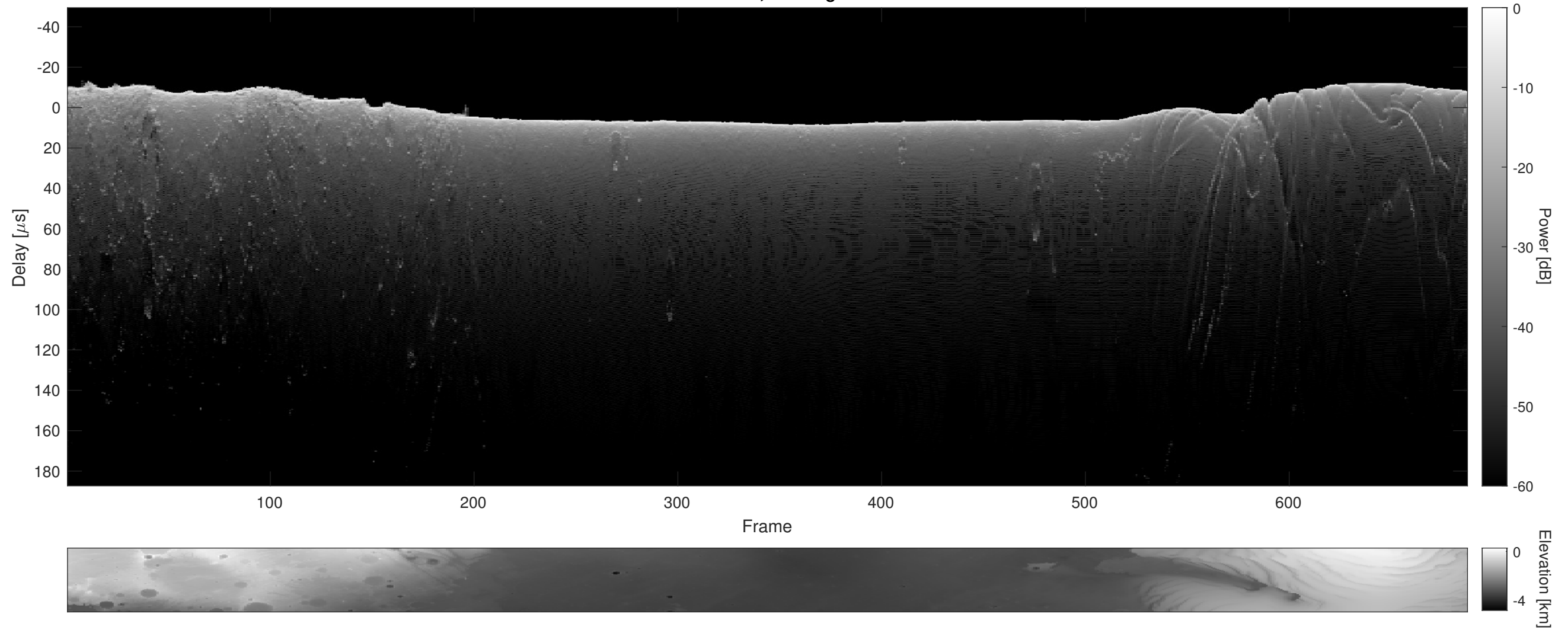
Orbit 22393, Cluttergram
