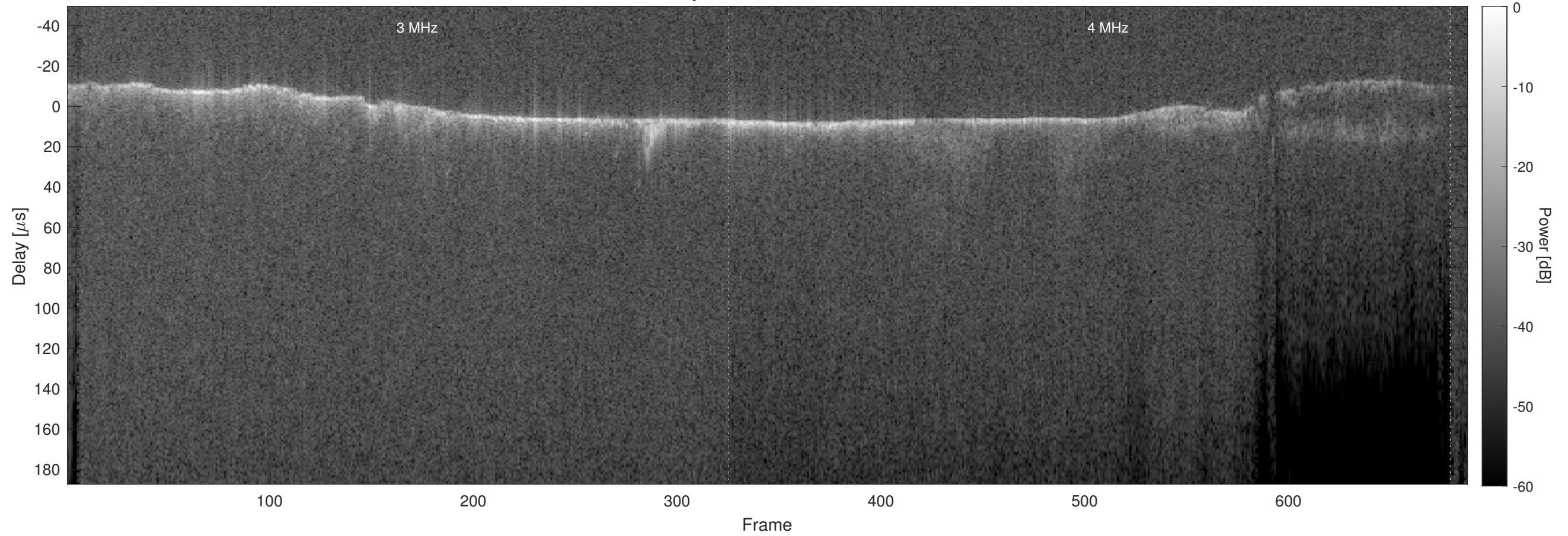
Orbit 22393, Optimized, No Window, Channel 2
