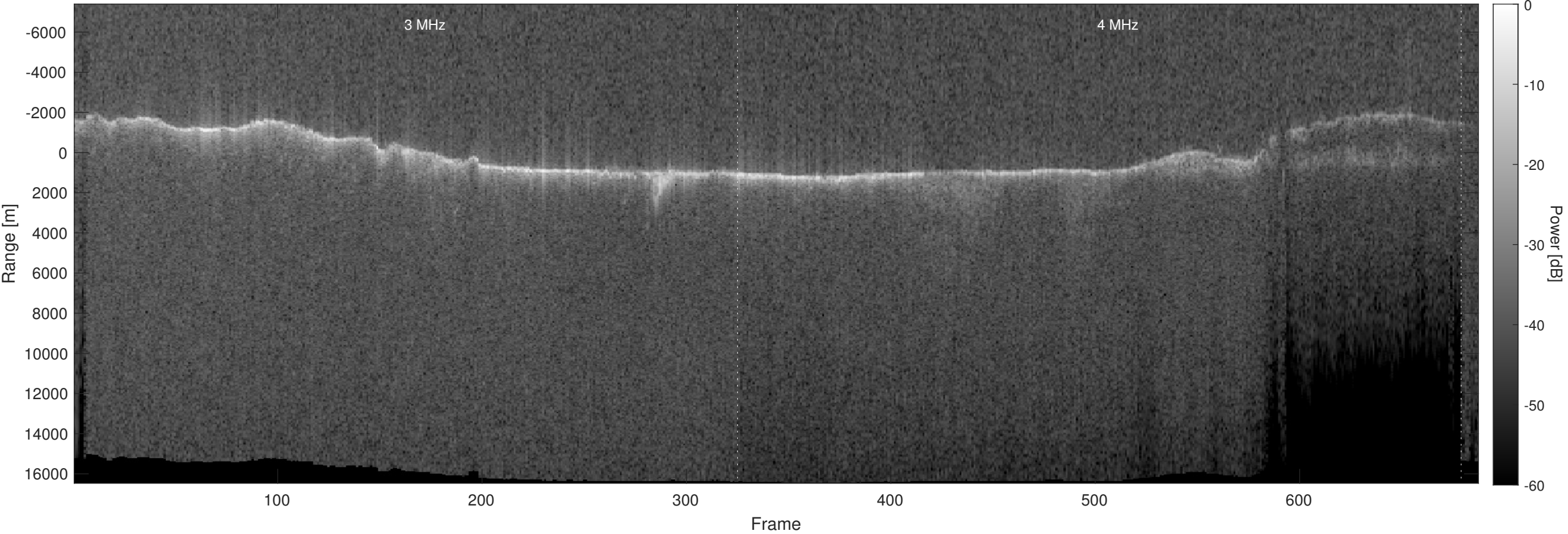
Orbit 22393, Optimized, No Window, Depth-Corrected, Channel 2
