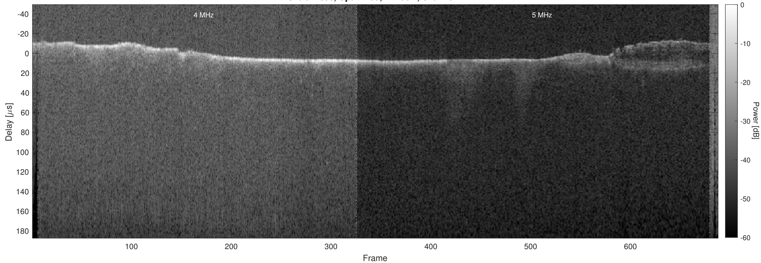
Orbit 22393, Optimized, Window, Channel 2
