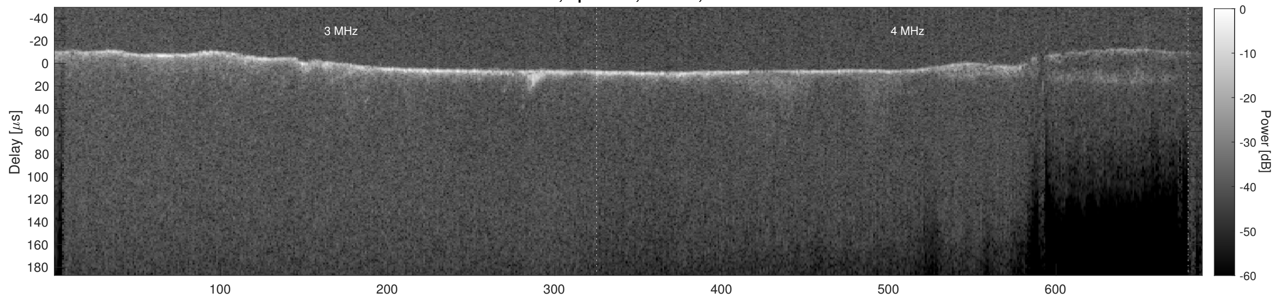
Orbit 22393, Cluttergram
