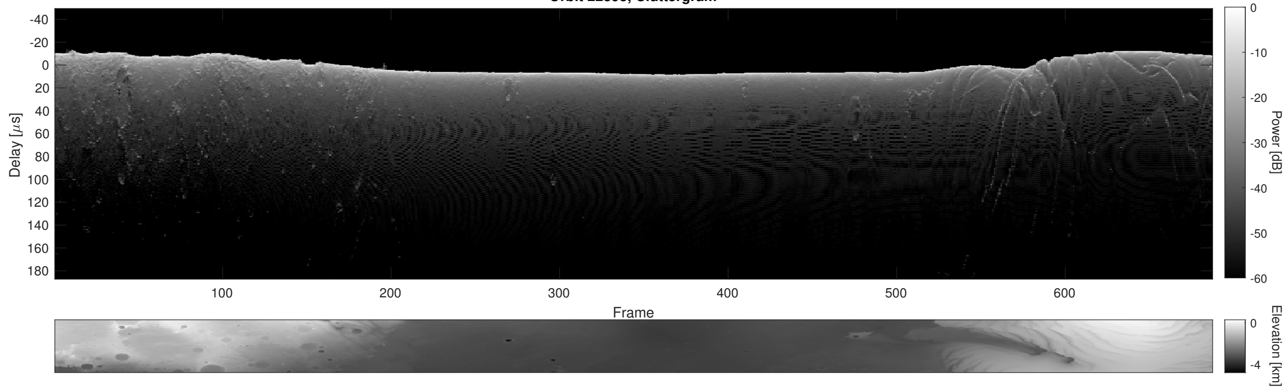
Orbit 22393, Cluttergram
