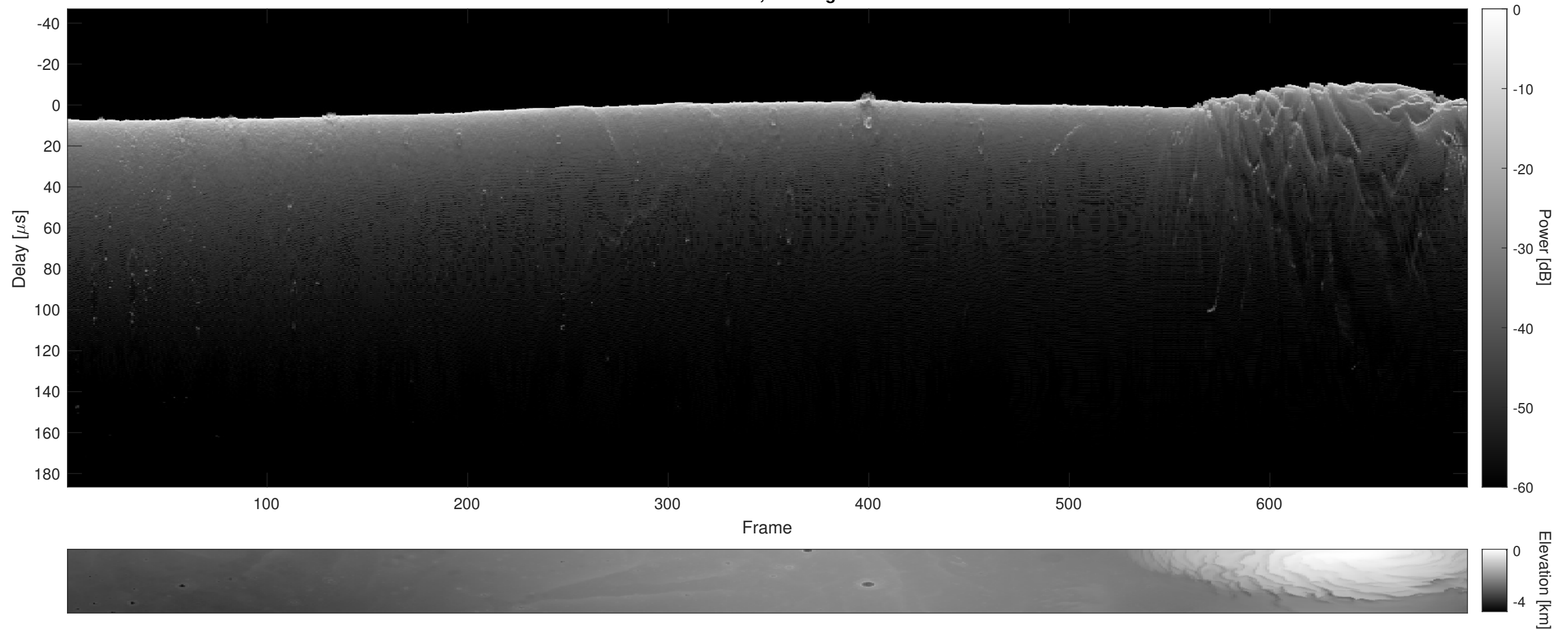
Orbit 22395, Cluttergram
