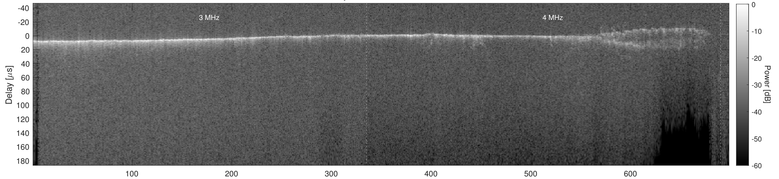
Orbit 22395, Cluttergram
