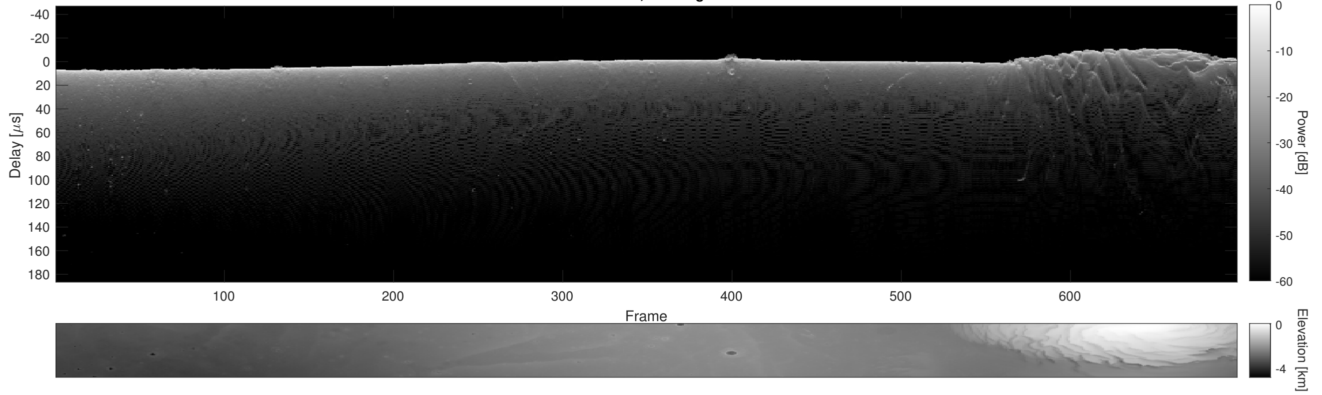
Orbit 22395, Cluttergram
