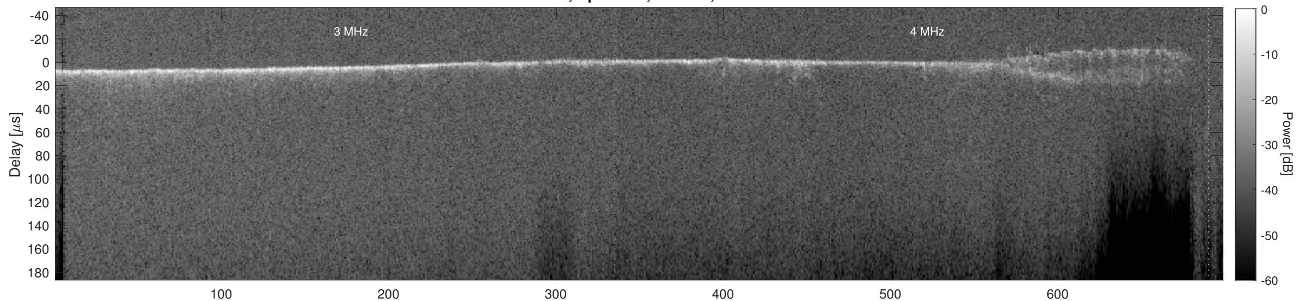
Orbit 22395, Cluttergram
