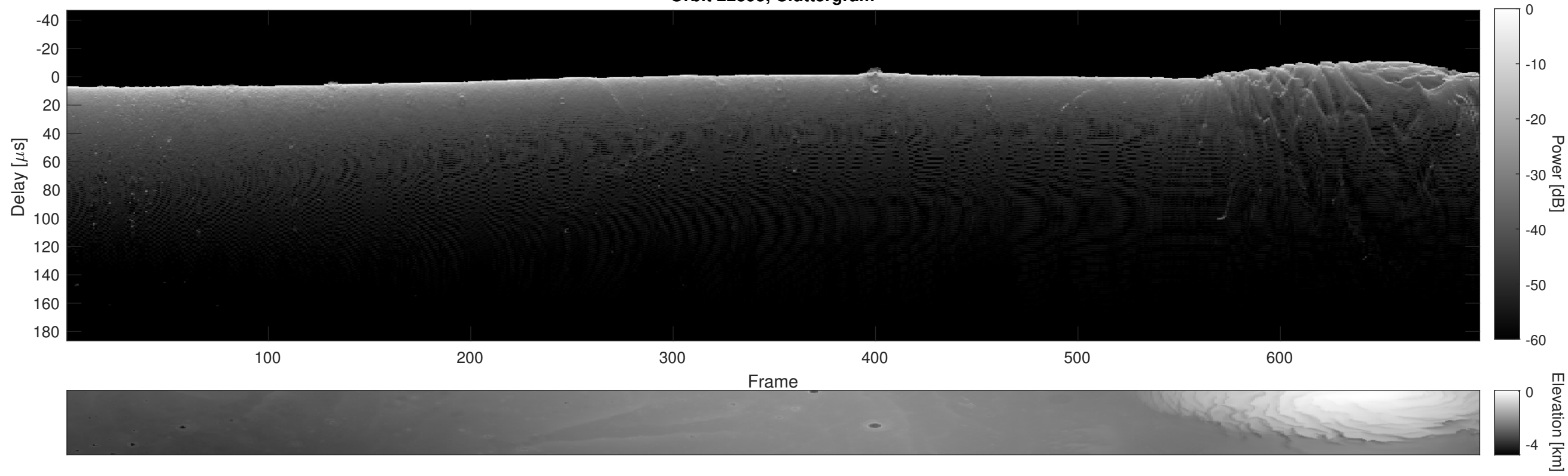
Orbit 22395, Cluttergram
