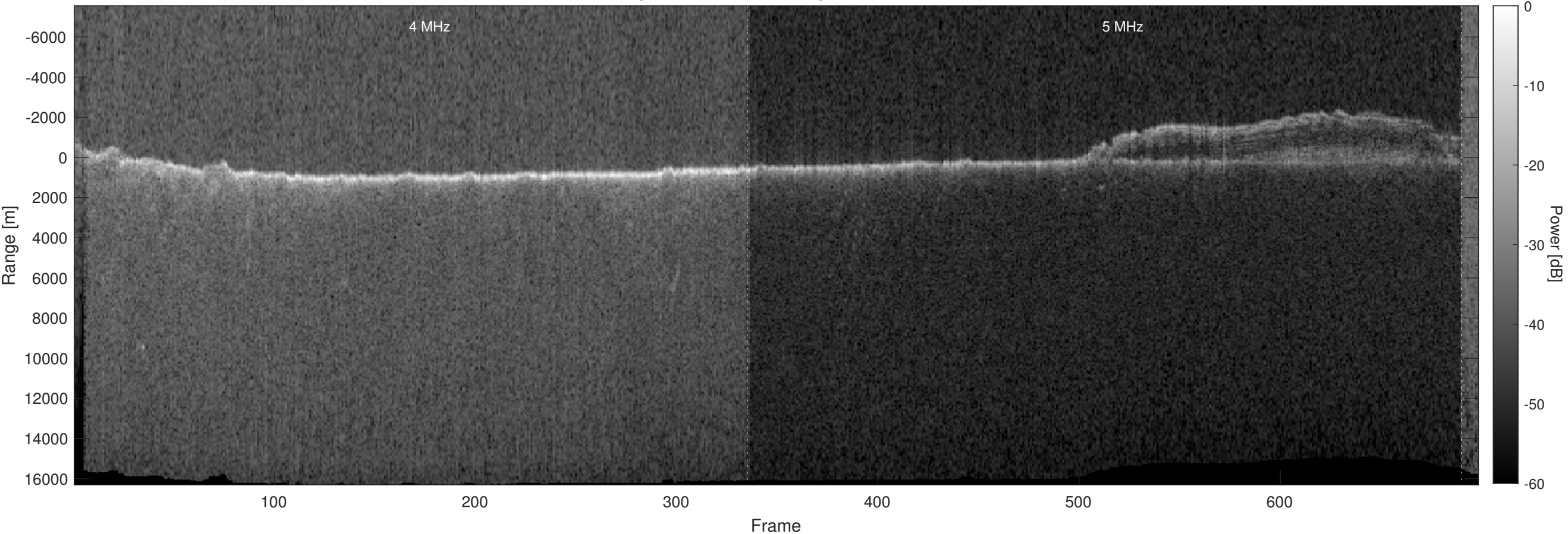
Orbit 22396, Optimized, Window, Depth-Corrected, Channel 2
