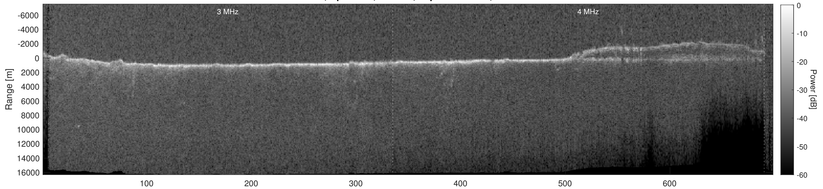
Orbit 22396, Depth-Corrected Cluttergram
