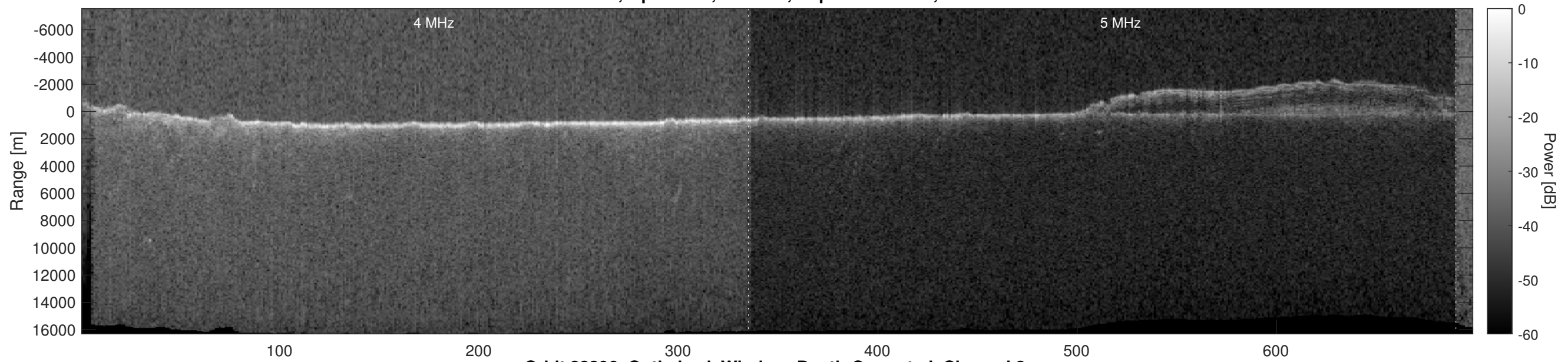
Orbit 22396, Optimized, Window, Depth-Corrected, Channel 2
