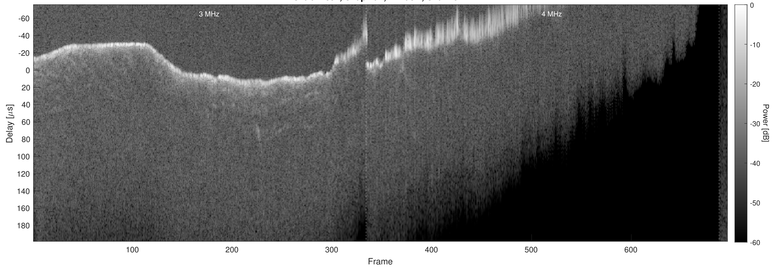
Orbit 22397, Chapman, Window, Channel 2
