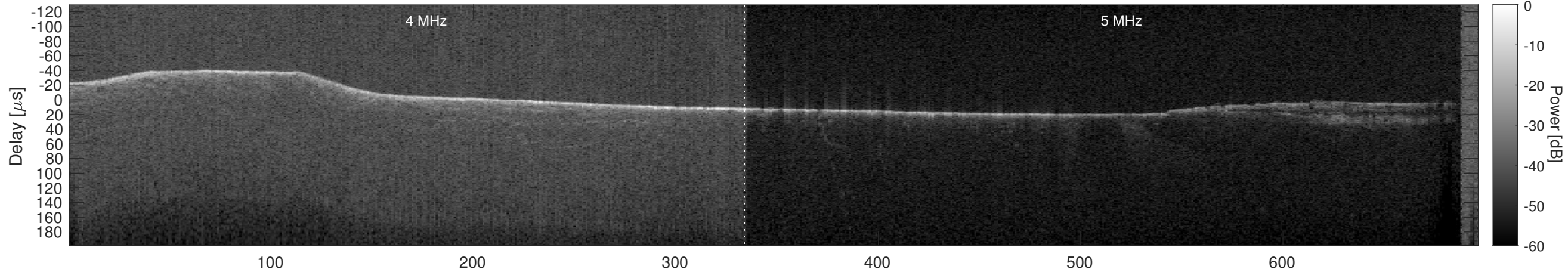
Orbit 22397, Cluttergram
