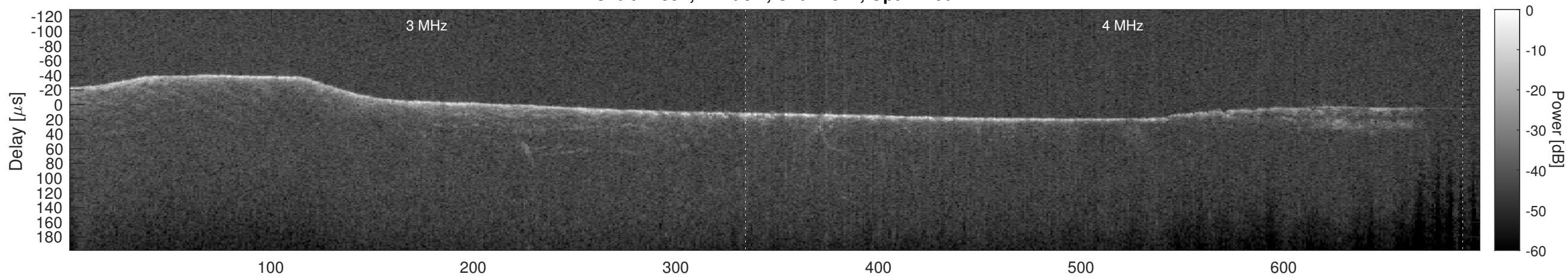
Orbit 22397, Cluttergram
