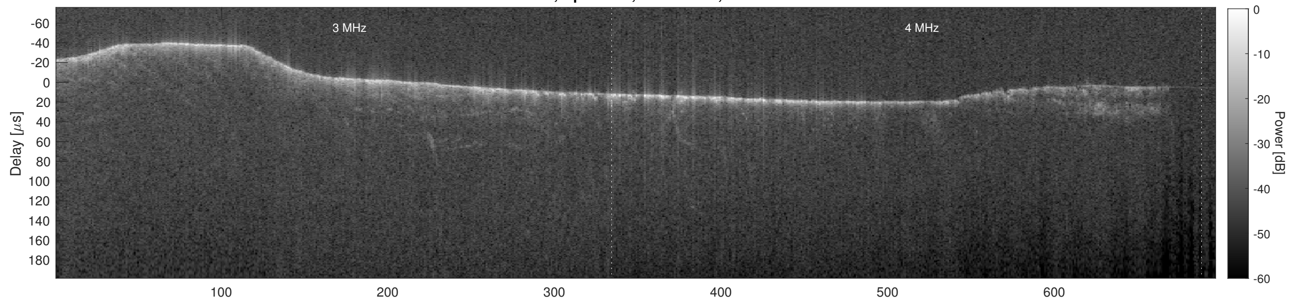
Orbit 22397, Cluttergram
