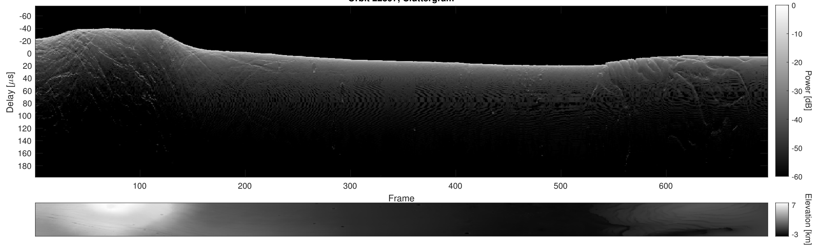
Orbit 22397, Cluttergram
