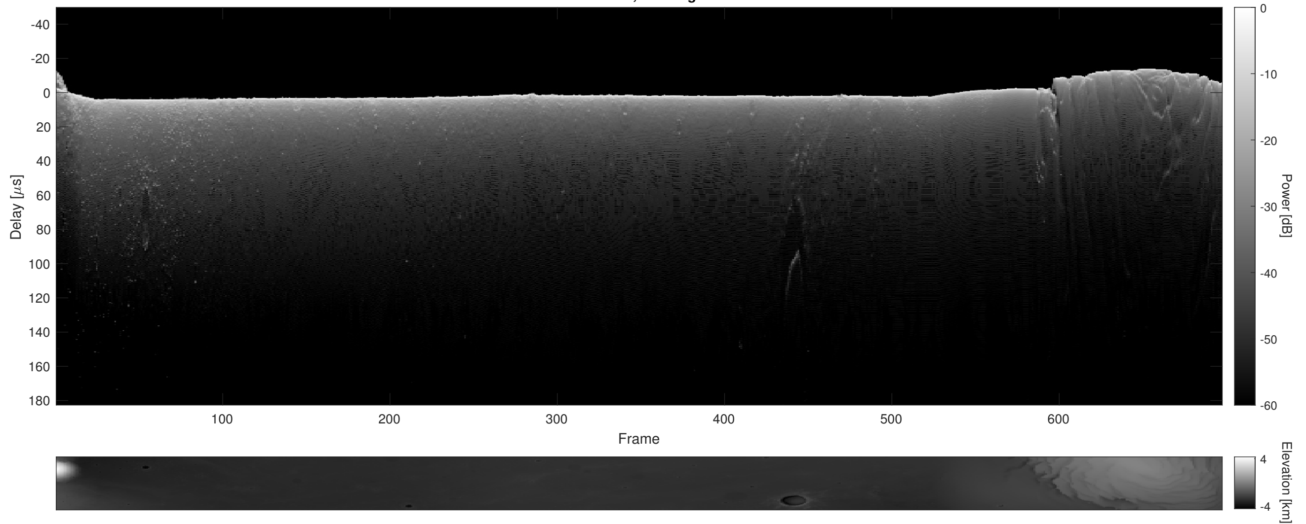
Orbit 22398, Cluttergram
