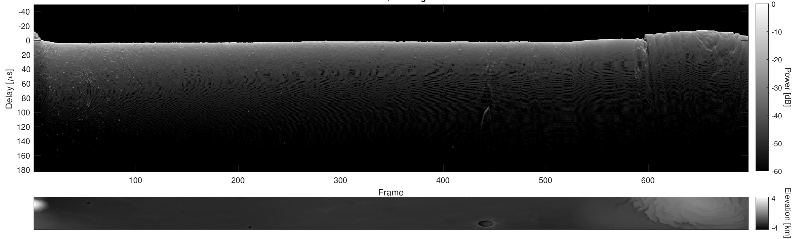
Orbit 22398, Cluttergram
