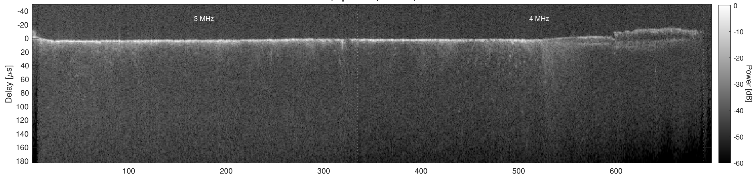
Orbit 22398, Cluttergram
