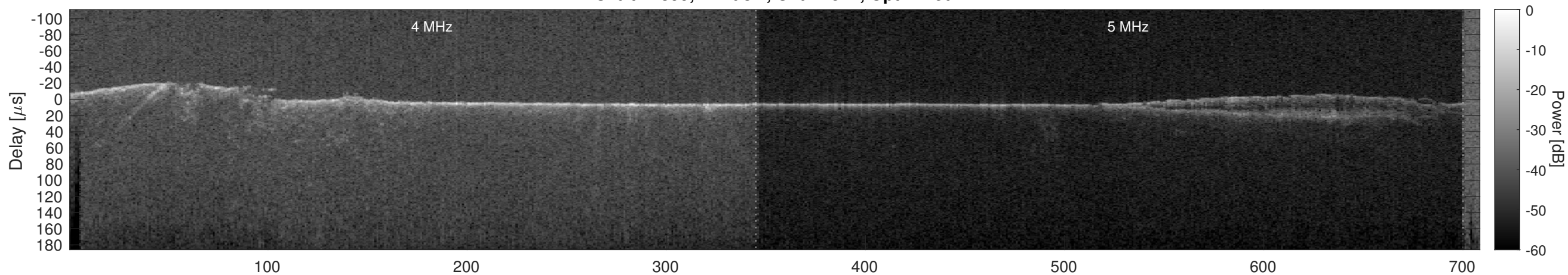
Orbit 22399, Cluttergram
