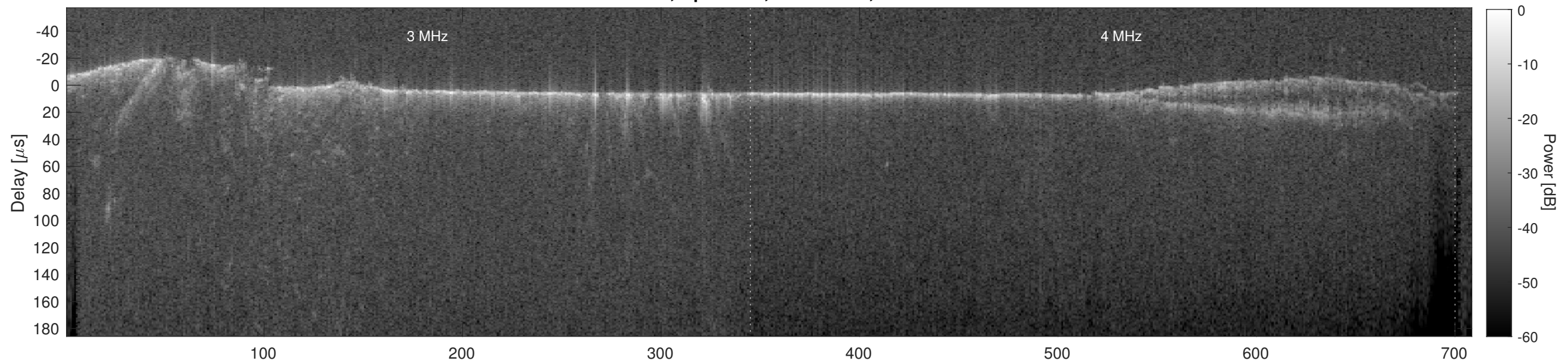
Orbit 22399, Cluttergram
