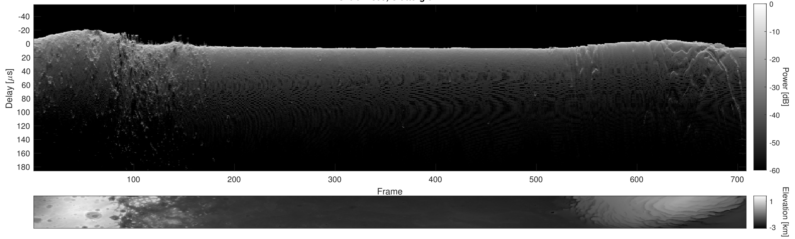
Orbit 22399, Cluttergram
