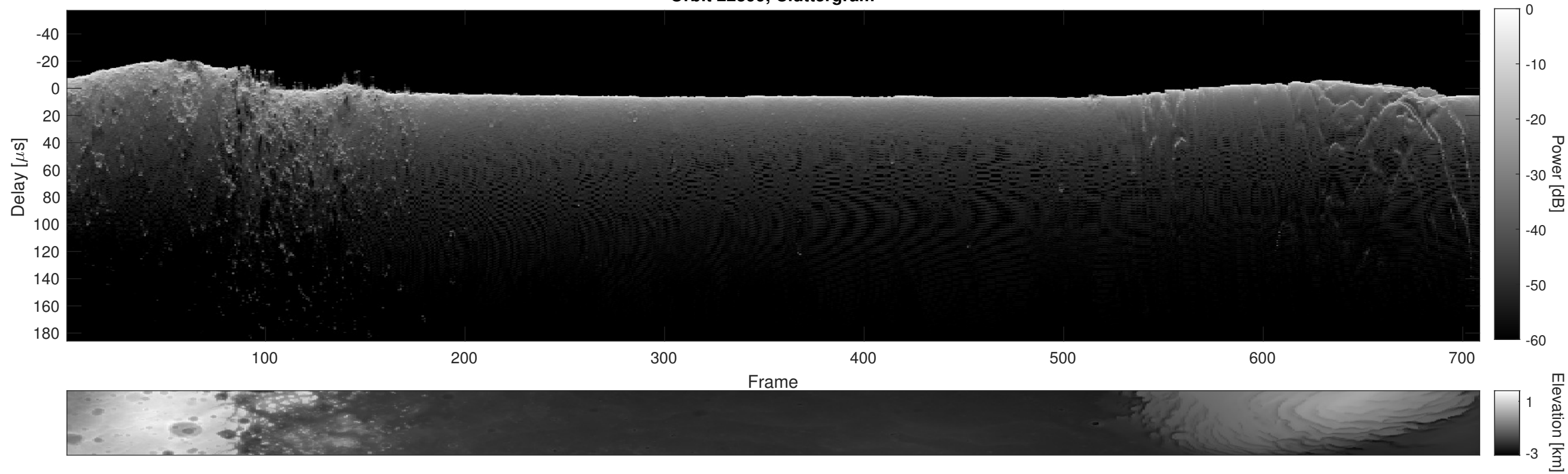
Orbit 22399, Cluttergram
