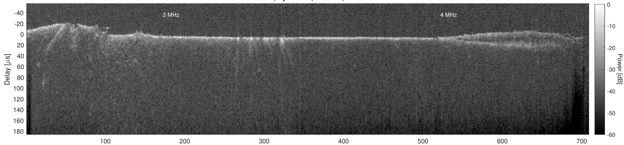
Orbit 22399, Cluttergram
