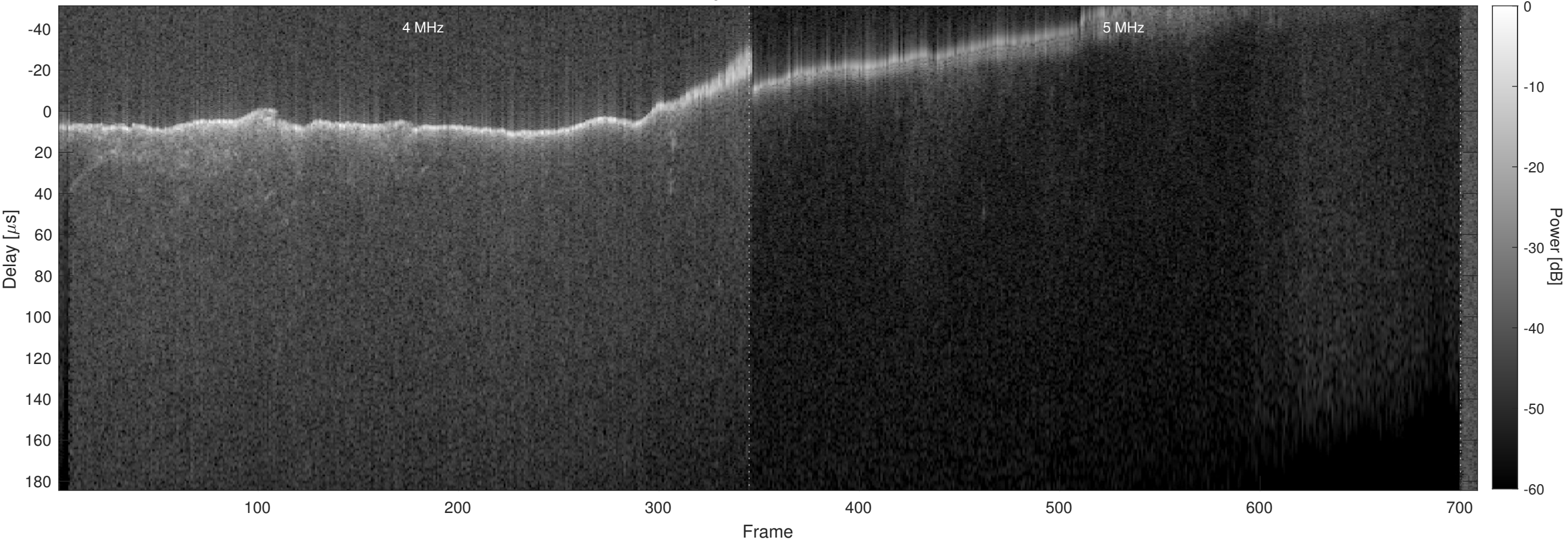
Orbit 22400, Chapman, No Window, Channel 2
