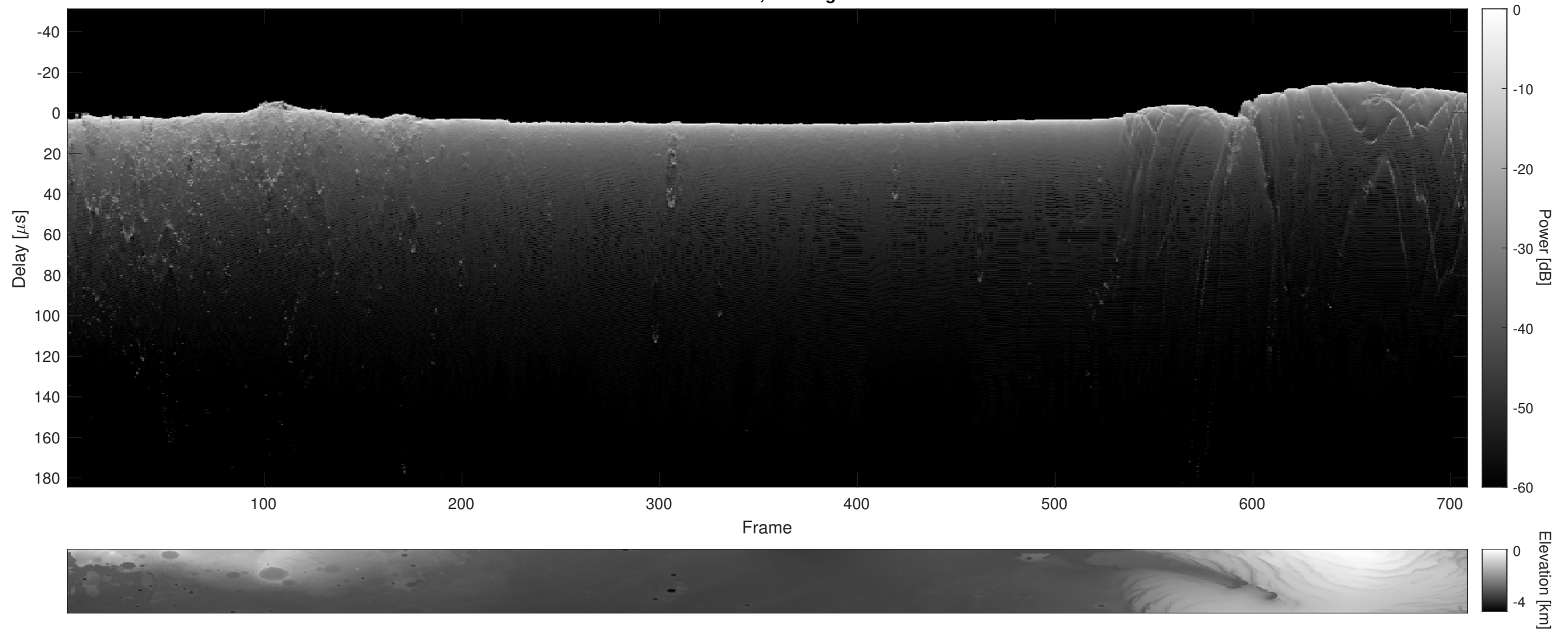
Orbit 22400, Cluttergram
