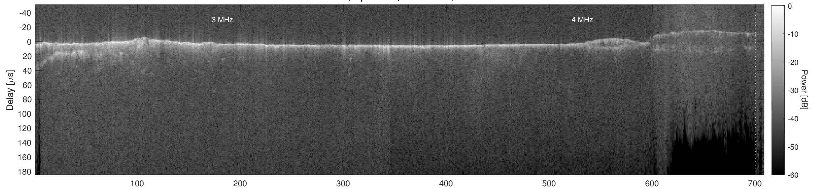
Orbit 22400, Cluttergram
