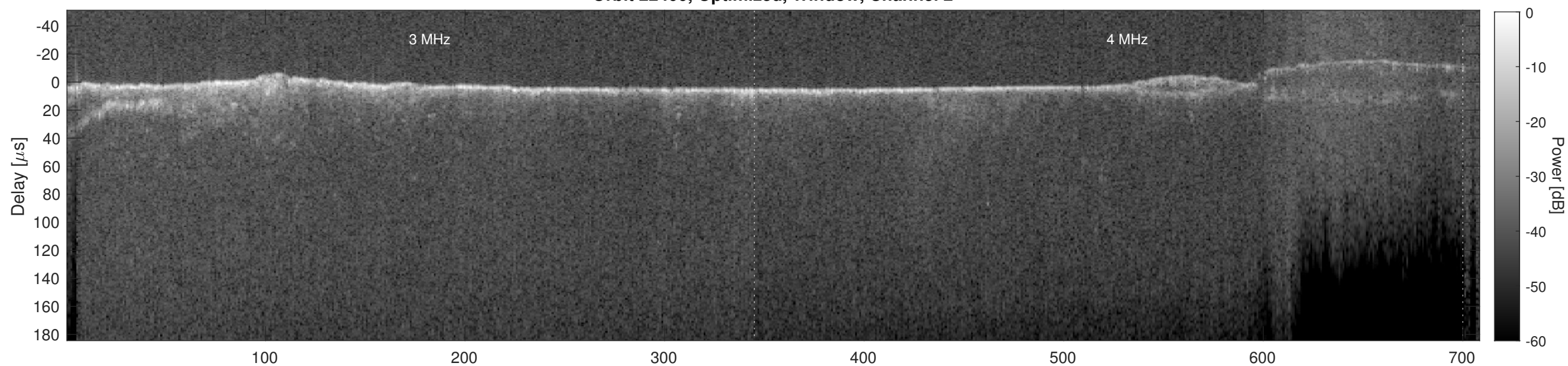
Orbit 22400, Cluttergram
