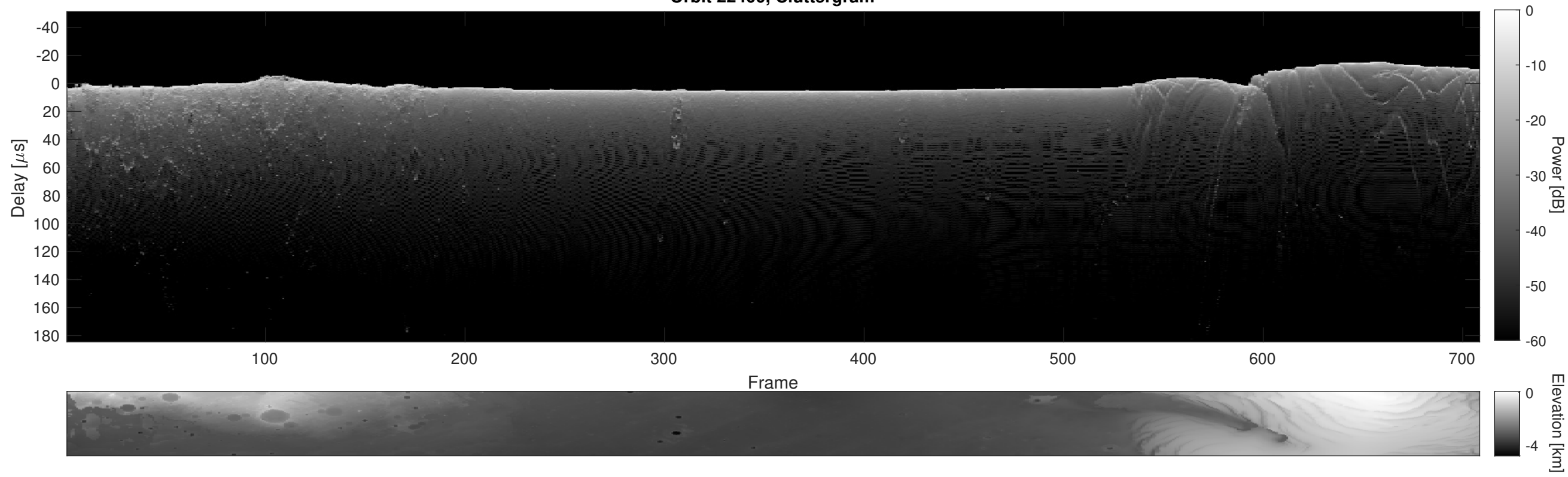
Orbit 22400, Cluttergram
