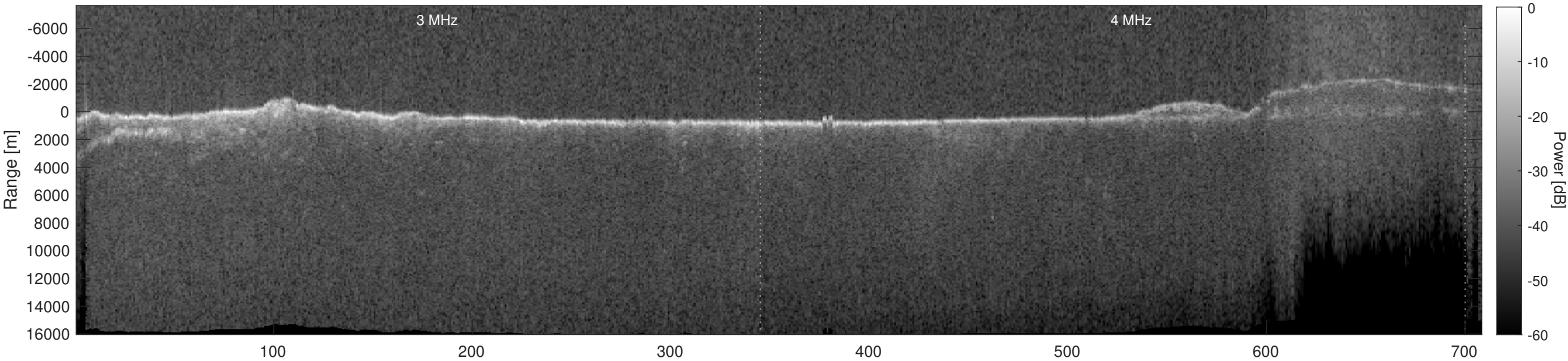
Orbit 22400, Depth-Corrected Cluttergram
