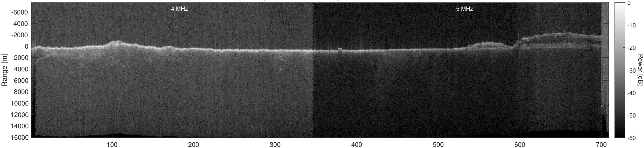
Orbit 22400, Optimized, Window, Depth-Corrected, Channel 2
