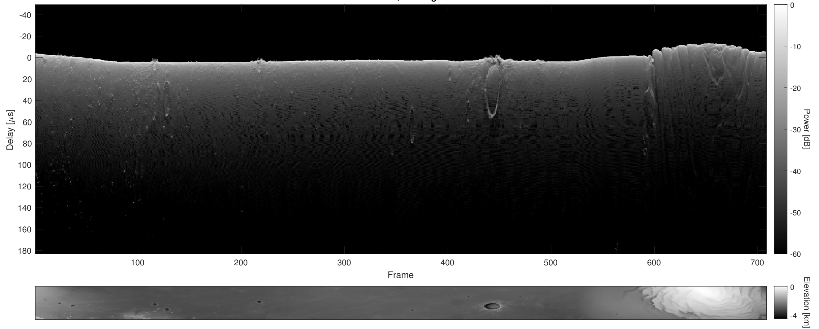
Orbit 22405, Cluttergram
