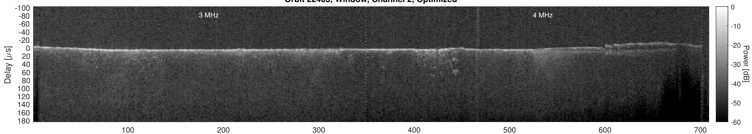
Orbit 22405, Cluttergram
