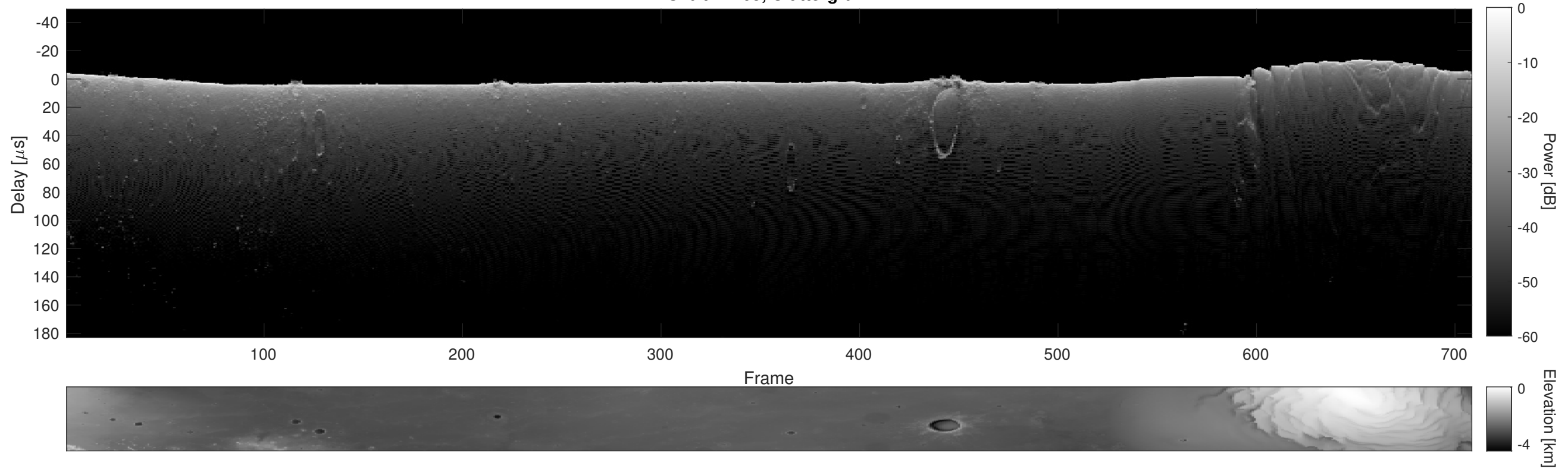
Orbit 22405, Cluttergram
