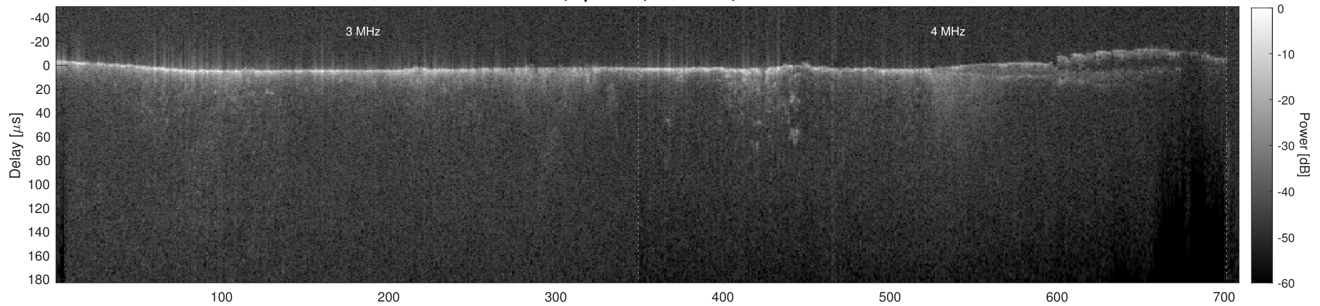
Orbit 22405, Cluttergram
