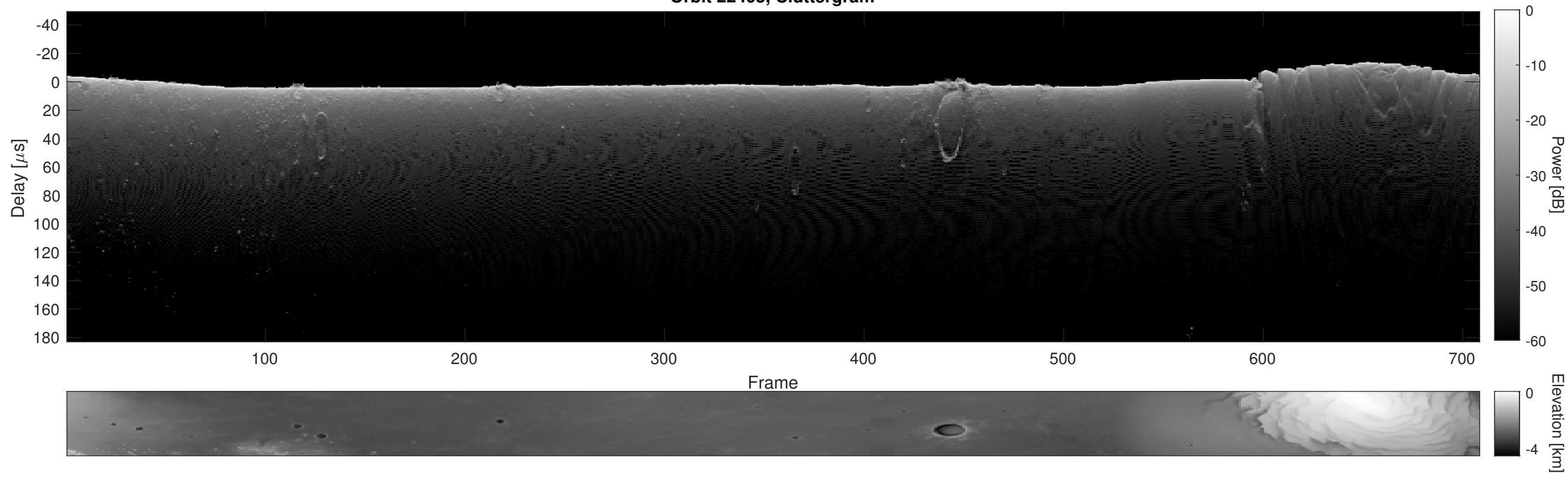
Orbit 22405, Cluttergram
