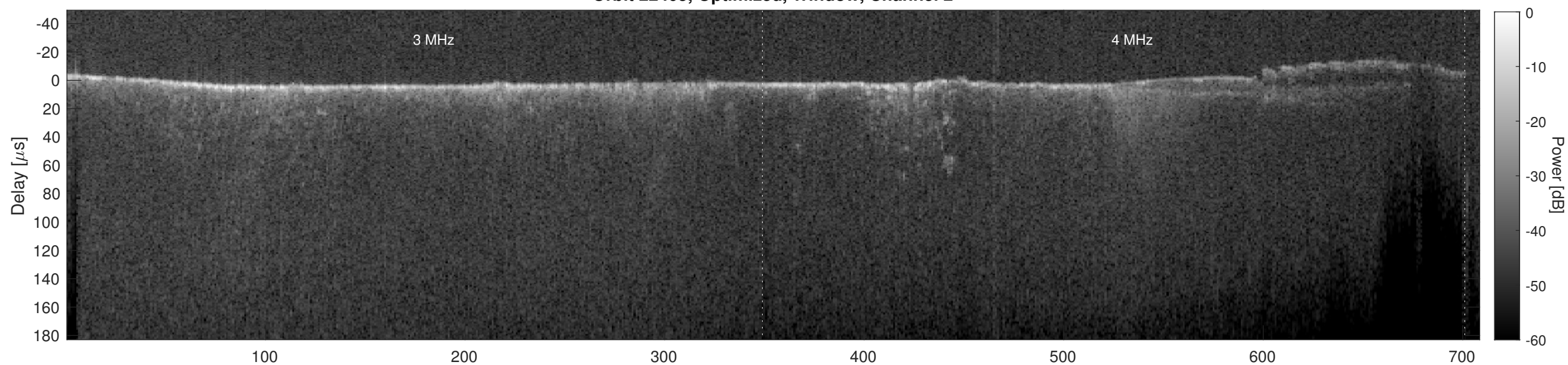
Orbit 22405, Cluttergram
